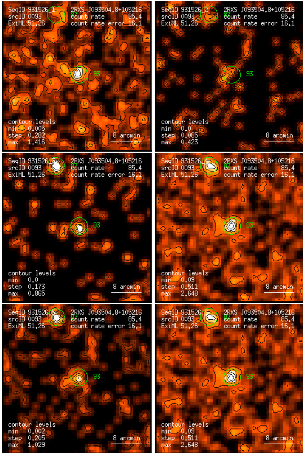
Figure 93: RASS 931526: detection 0093: band rate images, Gaussian filter: (1) PSPC channels 11 – 41, (2) 52 – 90, (3) 91 – 201, (4) 11 – 235, (5) 52 – 201, (6) 11 – 201. Broad band rates in counts/ks. Band rate contour levels in counts/ks/arcmin 2 .
