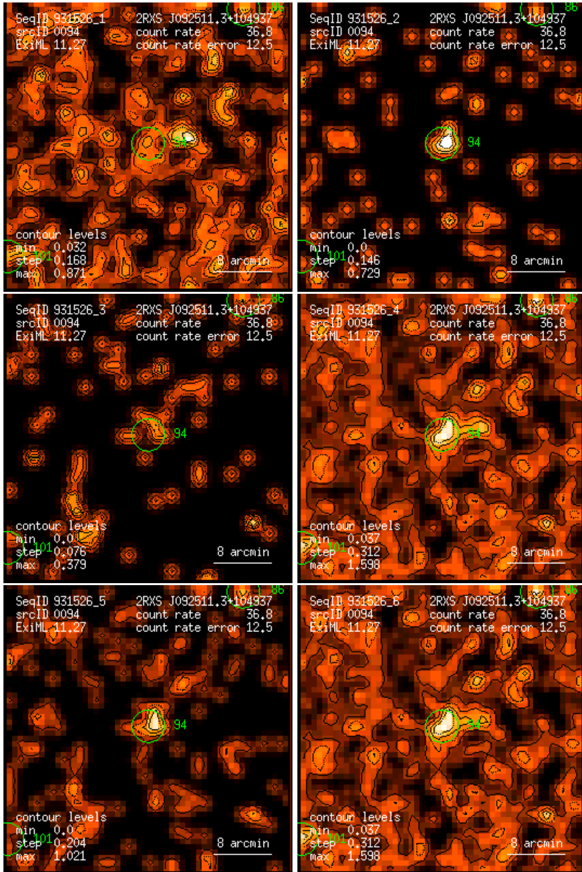
Figure 94: RASS 931526: detection 0094: band rate images, Gaussian filter: (1) PSPC channels 11 – 41, (2) 52 – 90, (3) 91 – 201, (4) 11 – 235, (5) 52 – 201, (6) 11 – 201. Broad band rates in counts/ks. Band rate contour levels in counts/ks/arcmin 2 .
