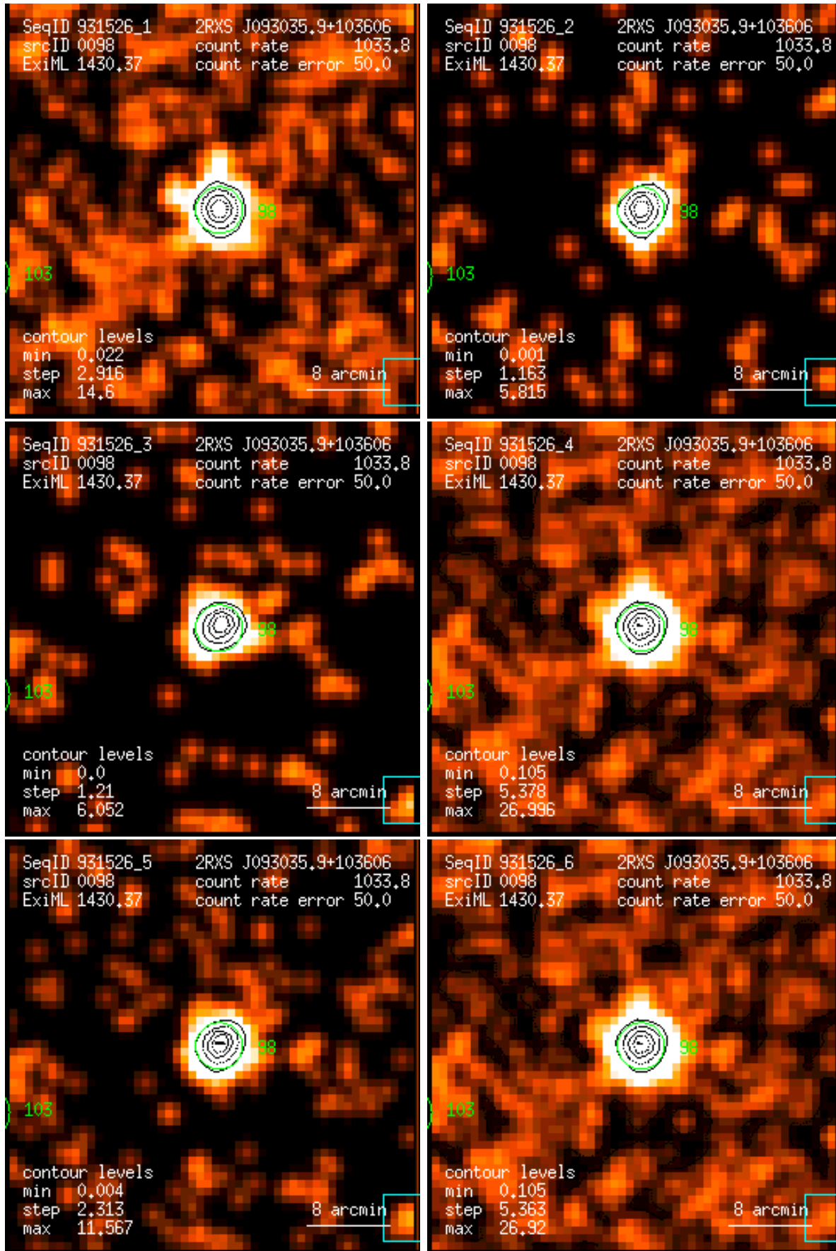
Figure 98: RASS 931526: detection 0098: band rate images, Gaussian filter: (1) PSPC channels 11 – 41, (2) 52 – 90, (3) 91 – 201, (4) 11 – 235, (5) 52 – 201, (6) 11 – 201. Broad band rates in counts/ks. Band rate contour levels in counts/ks/arcmin 2 .
