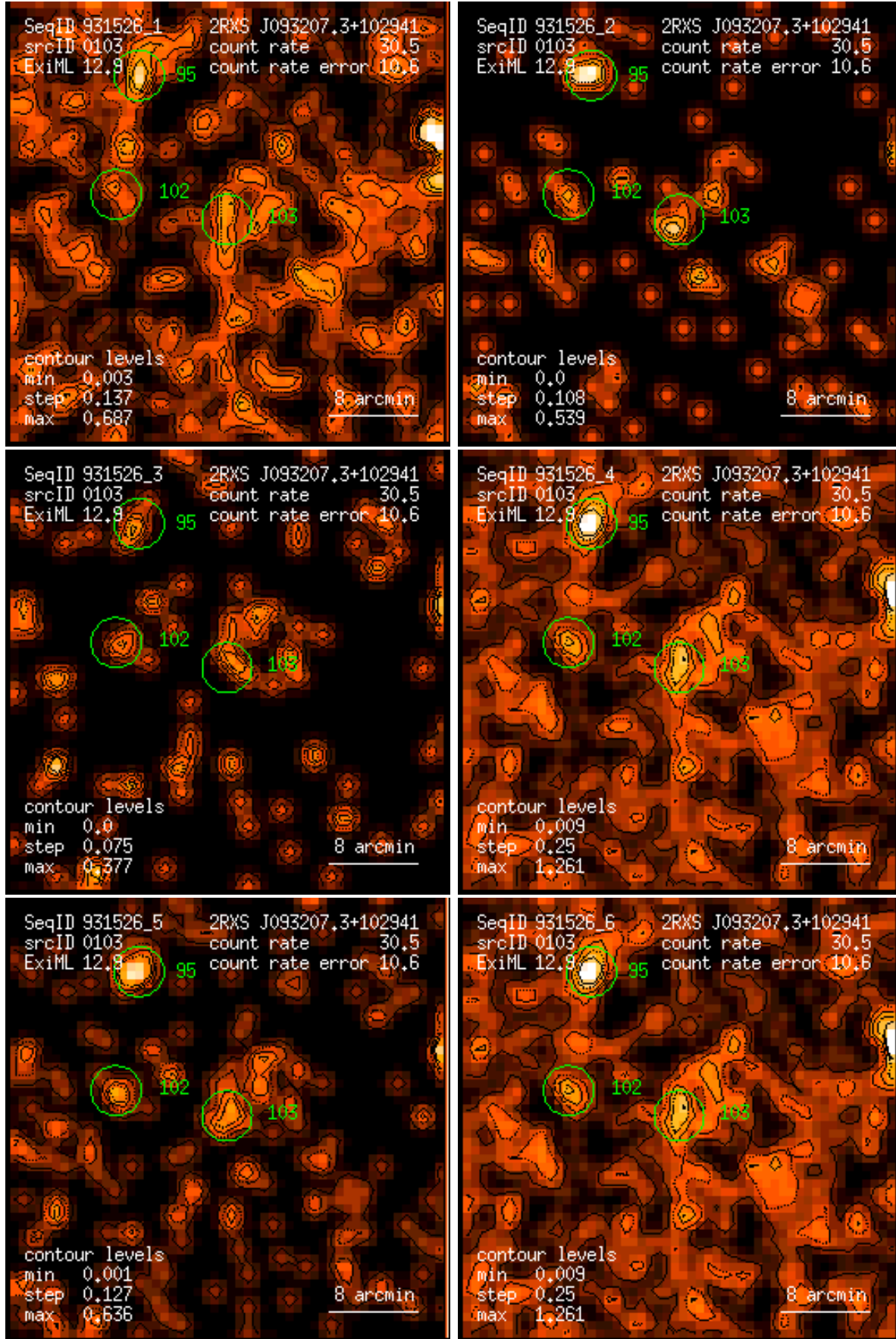
Figure 103: RASS 931526: detection 0103: band rate images, Gaussian filter: (1) PSPC channels 11 – 41, (2) 52 – 90, (3) 91 – 201, (4) 11 – 235, (5) 52 – 201, (6) 11 – 201. Broad band rates in counts/ks. Band rate contour levels in counts/ks/arcmin 2 .
