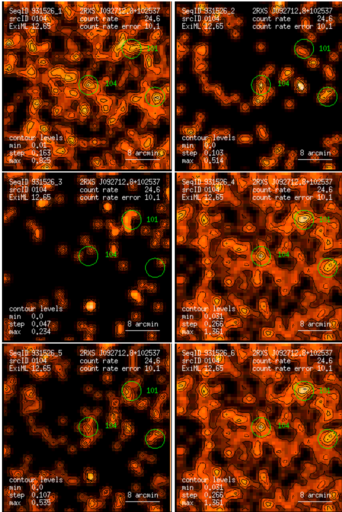
Figure 104: RASS 931526: detection 0104: band rate images, Gaussian filter: (1) PSPC channels 11 – 41, (2) 52 – 90, (3) 91 – 201, (4) 11 – 235, (5) 52 – 201, (6) 11 – 201. Broad band rates in counts/ks. Band rate contour levels in counts/ks/arcmin 2 .
