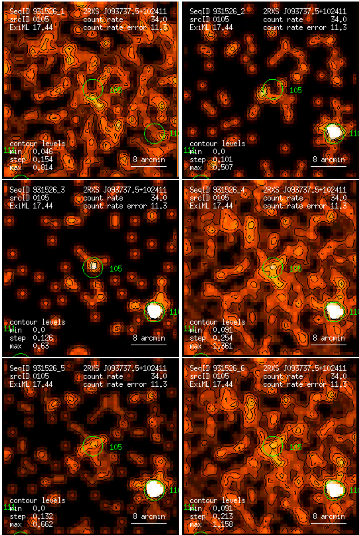
Figure 105: RASS 931526: detection 0105: band rate images, Gaussian filter: (1) PSPC channels 11 – 41, (2) 52 – 90, (3) 91 – 201, (4) 11 – 235, (5) 52 – 201, (6) 11 – 201. Broad band rates in counts/ks. Band rate contour levels in counts/ks/arcmin 2 .
