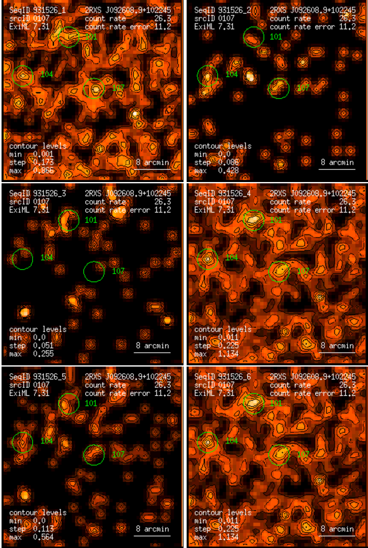
Figure 107: RASS 931526: detection 0107: band rate images, Gaussian filter: (1) PSPC channels 11 – 41, (2) 52 – 90, (3) 91 – 201, (4) 11 – 235, (5) 52 – 201, (6) 11 – 201. Broad band rates in counts/ks. Band rate contour levels in counts/ks/arcmin 2 .
