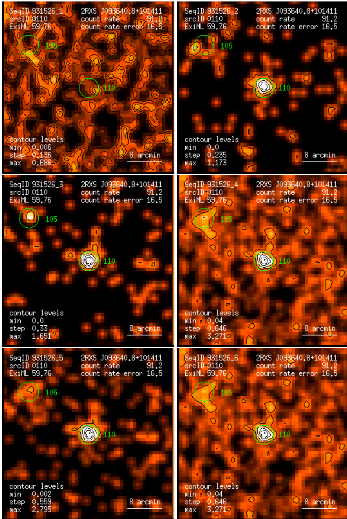
Figure 110: RASS 931526: detection 0110: band rate images, Gaussian filter: (1) PSPC channels 11 – 41, (2) 52 – 90, (3) 91 – 201, (4) 11 – 235, (5) 52 – 201, (6) 11 – 201. Broad band rates in counts/ks. Band rate contour levels in counts/ks/arcmin 2 .
