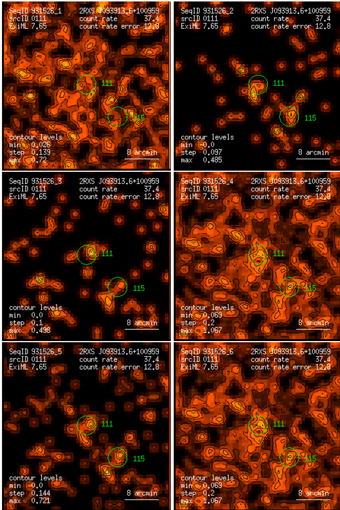
Figure 111: RASS 931526: detection 0111: band rate images, Gaussian filter: (1) PSPC channels 11 – 41, (2) 52 – 90, (3) 91 – 201, (4) 11 – 235, (5) 52 – 201, (6) 11 – 201. Broad band rates in counts/ks. Band rate contour levels in counts/ks/arcmin 2 .
