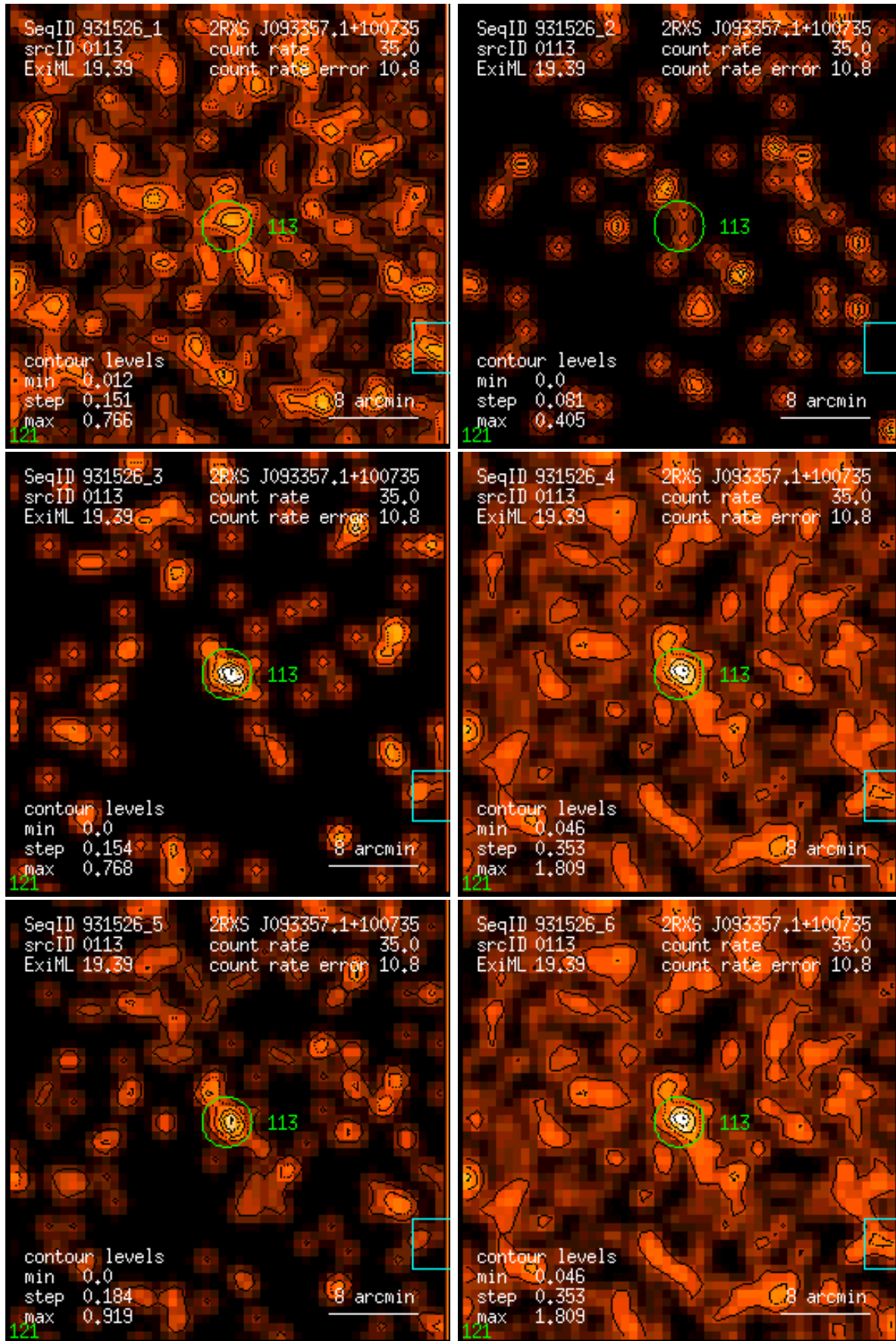
Figure 113: RASS 931526: detection 0113: band rate images, Gaussian filter: (1) PSPC channels 11 – 41, (2) 52 – 90, (3) 91 – 201, (4) 11 – 235, (5) 52 – 201, (6) 11 – 201. Broad band rates in counts/ks. Band rate contour levels in counts/ks/arcmin 2 .
