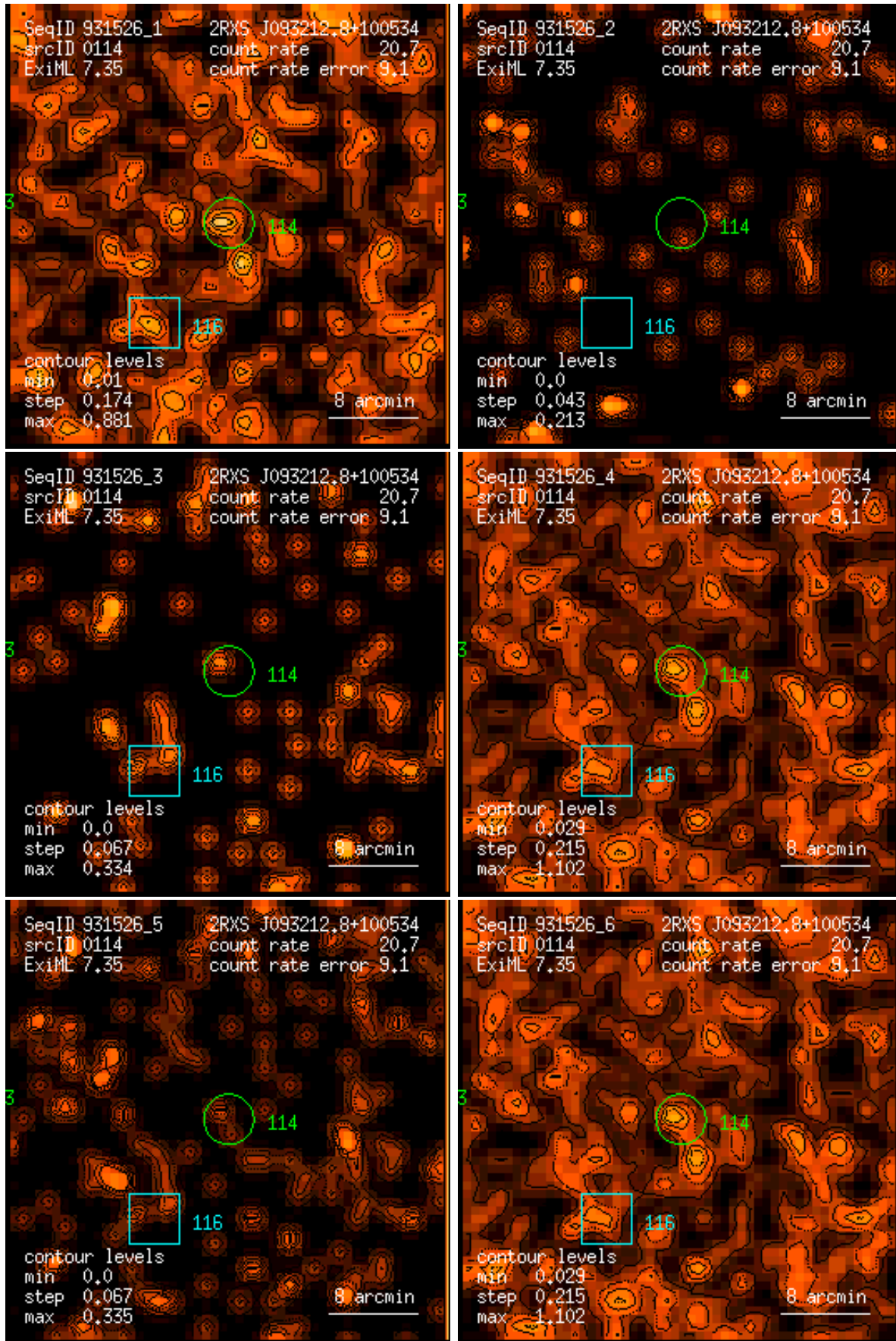
Figure 114: RASS 931526: detection 0114: band rate images, Gaussian filter: (1) PSPC channels 11 – 41, (2) 52 – 90, (3) 91 – 201, (4) 11 – 235, (5) 52 – 201, (6) 11 – 201. Broad band rates in counts/ks. Band rate contour levels in counts/ks/arcmin 2 .
