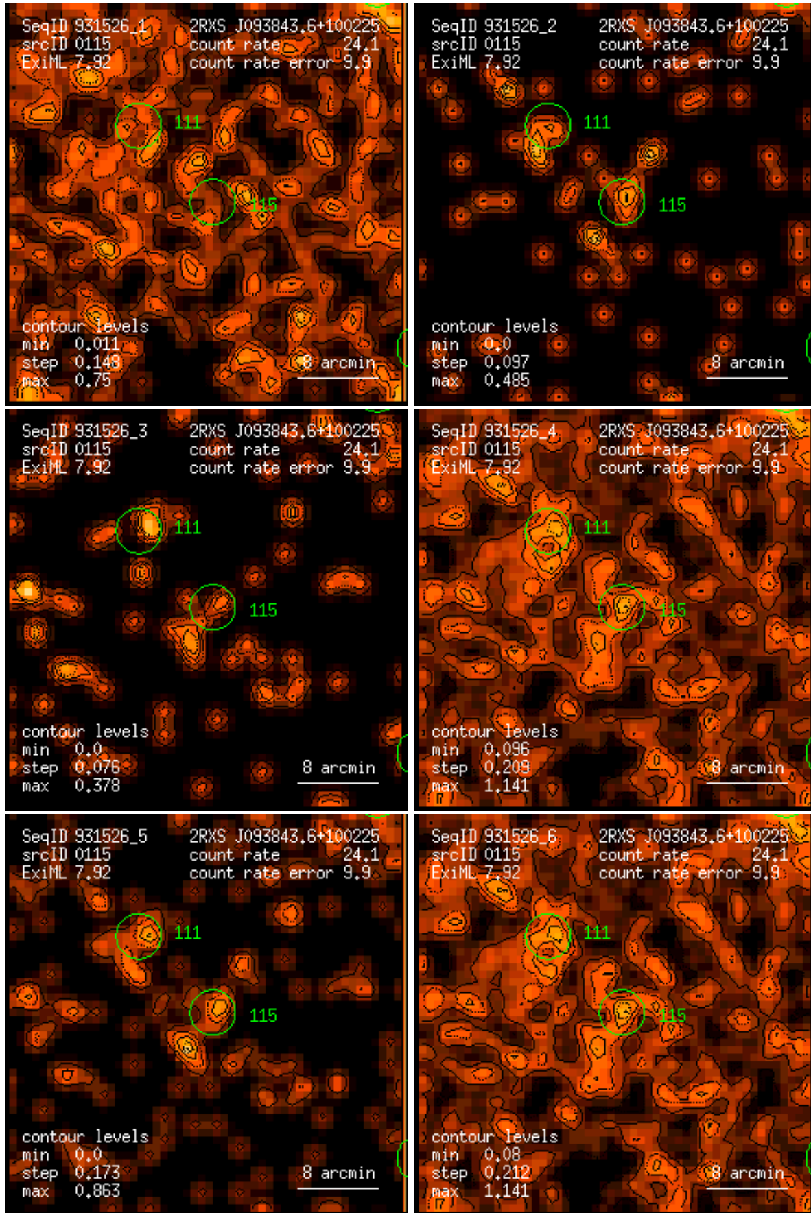
Figure 115: RASS 931526: detection 0115: band rate images, Gaussian filter: (1) PSPC channels 11 – 41, (2) 52 – 90, (3) 91 – 201, (4) 11 – 235, (5) 52 – 201, (6) 11 – 201. Broad band rates in counts/ks. Band rate contour levels in counts/ks/arcmin 2 .
