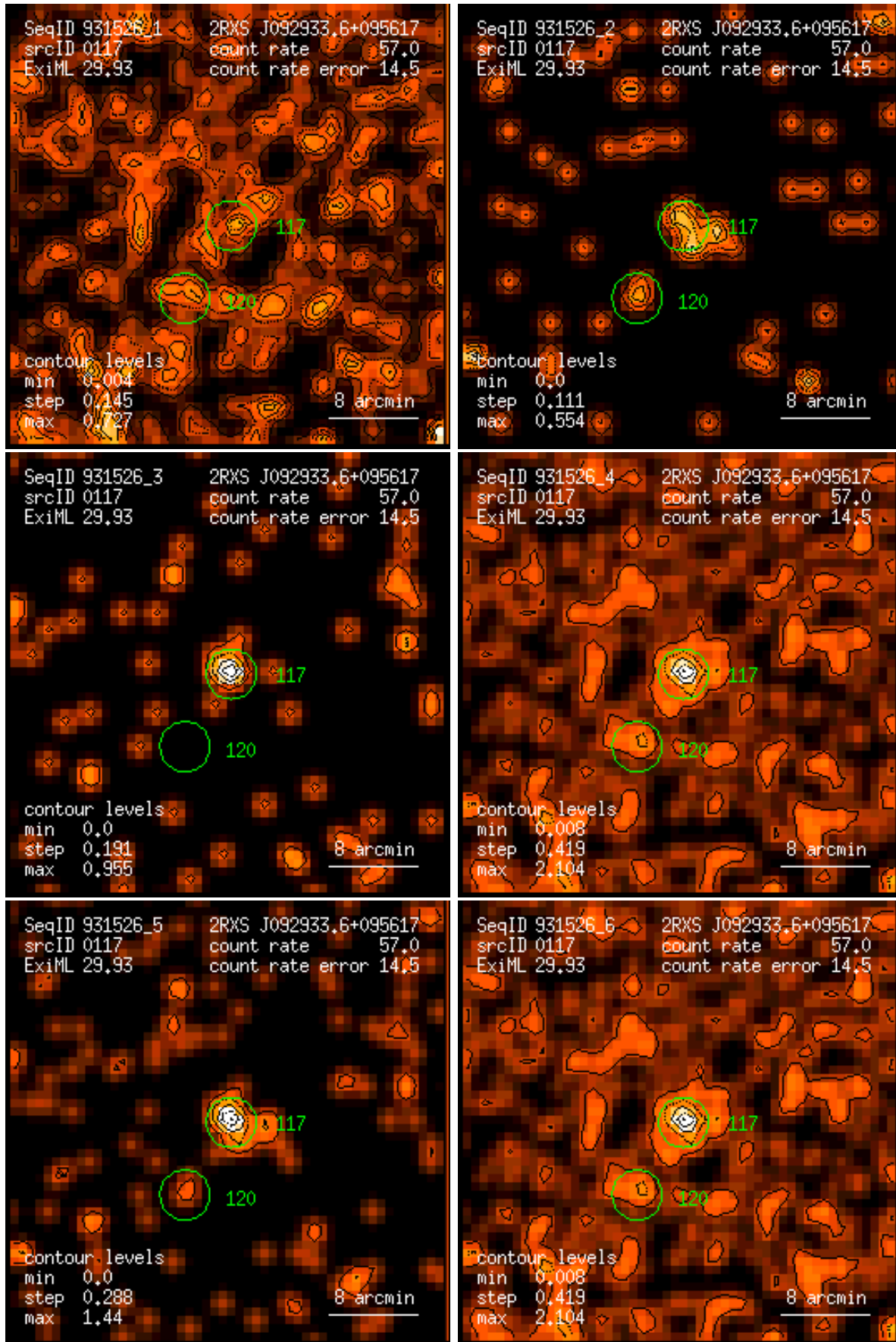
Figure 117: RASS 931526: detection 0117: band rate images, Gaussian filter: (1) PSPC channels 11 – 41, (2) 52 – 90, (3) 91 – 201, (4) 11 – 235, (5) 52 – 201, (6) 11 – 201. Broad band rates in counts/ks. Band rate contour levels in counts/ks/arcmin 2 .
