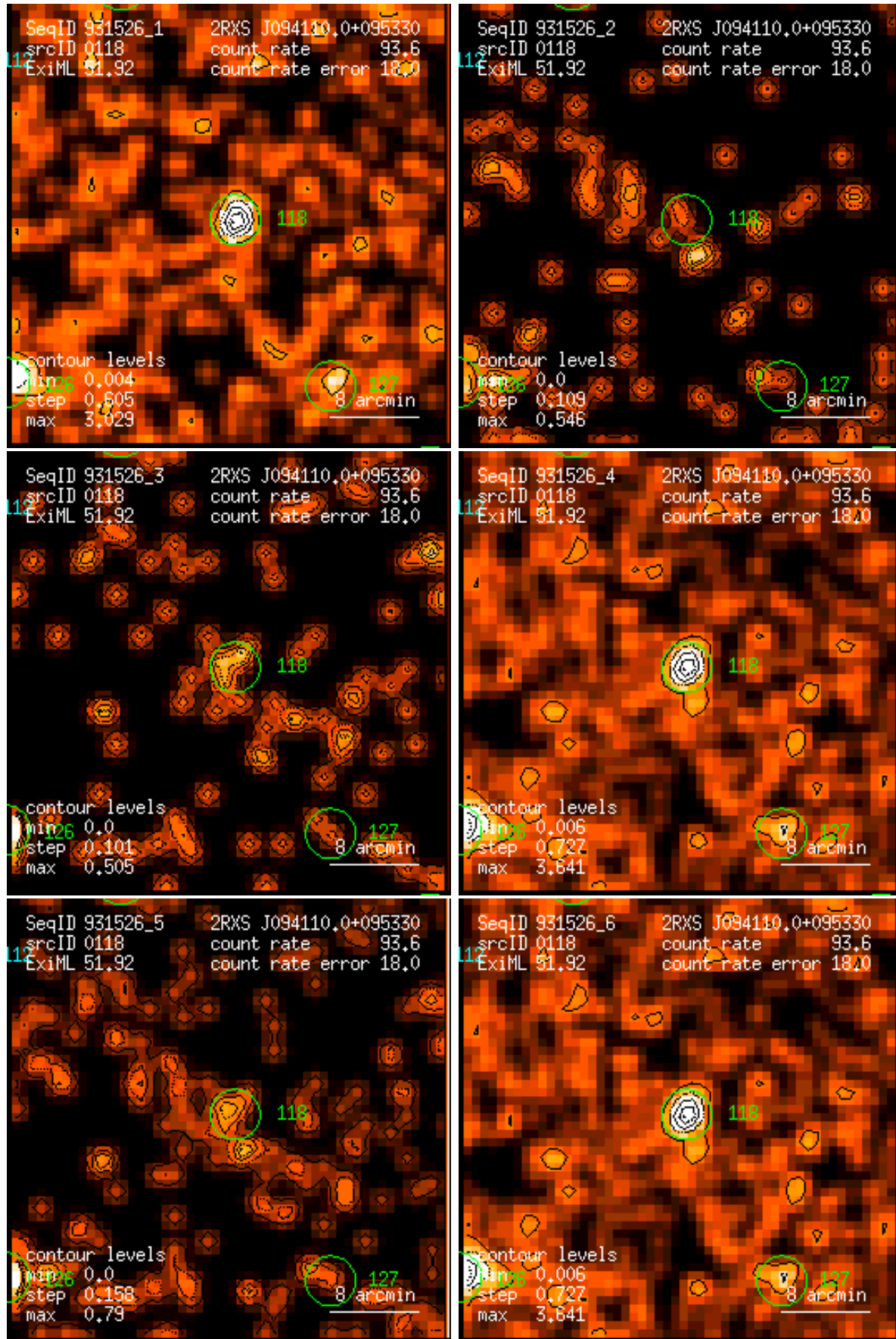
Figure 118: RASS 931526: detection 0118: band rate images, Gaussian filter: (1) PSPC channels 11 – 41, (2) 52 – 90, (3) 91 – 201, (4) 11 – 235, (5) 52 – 201, (6) 11 – 201. Broad band rates in counts/ks. Band rate contour levels in counts/ks/arcmin 2 .
