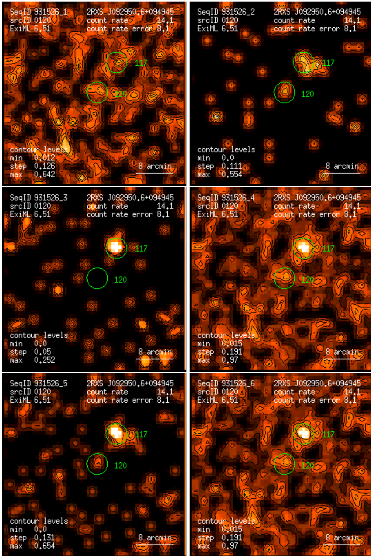
Figure 120: RASS 931526: detection 0120: band rate images, Gaussian filter: (1) PSPC channels 11 – 41, (2) 52 – 90, (3) 91 – 201, (4) 11 – 235, (5) 52 – 201, (6) 11 – 201. Broad band rates in counts/ks. Band rate contour levels in counts/ks/arcmin 2 .
