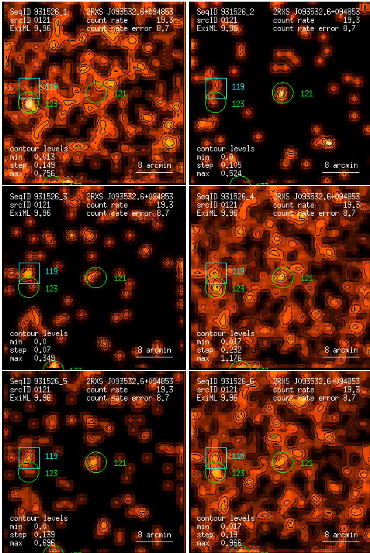
Figure 121: RASS 931526: detection 0121: band rate images, Gaussian filter: (1) PSCC channels 11 – 41, (2) 52 – 90, (3) 91 – 201, (4) 11 – 235, (5) 52 – 201, (6) 11 – 201. Broad band rates in counts/ks. Band rate contour levels in counts/ks/arcmin 2 .
