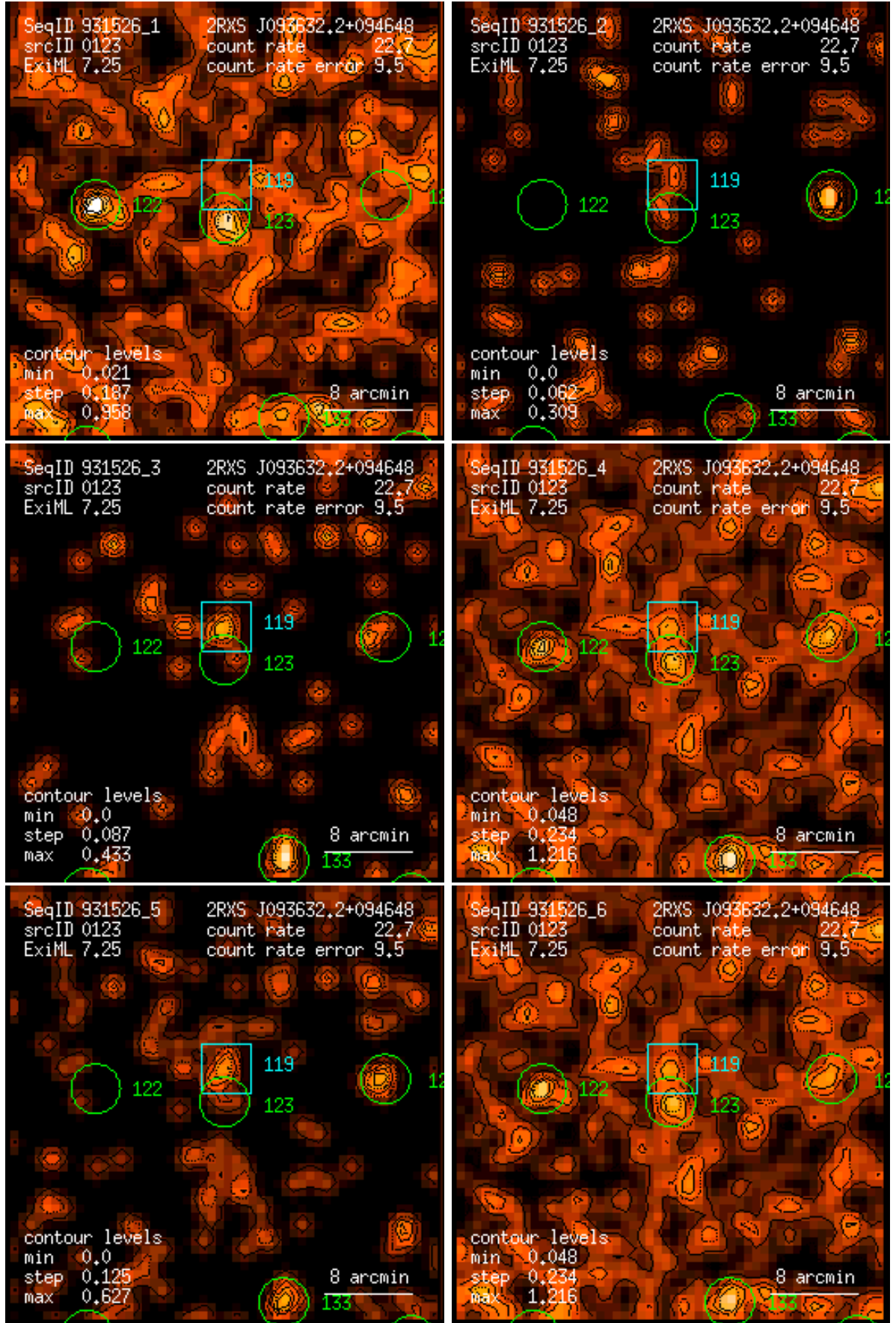
Figure 123: RASS 931526: detection 0123: band rate images, Gaussian filter: (1) PSPC channels 11 – 41, (2) 52 – 90, (3) 91 – 201, (4) 11 – 235, (5) 52 – 201, (6) 11 – 201. Broad band rates in counts/ks. Band rate contour levels in counts/ks/arcmin 2 .
