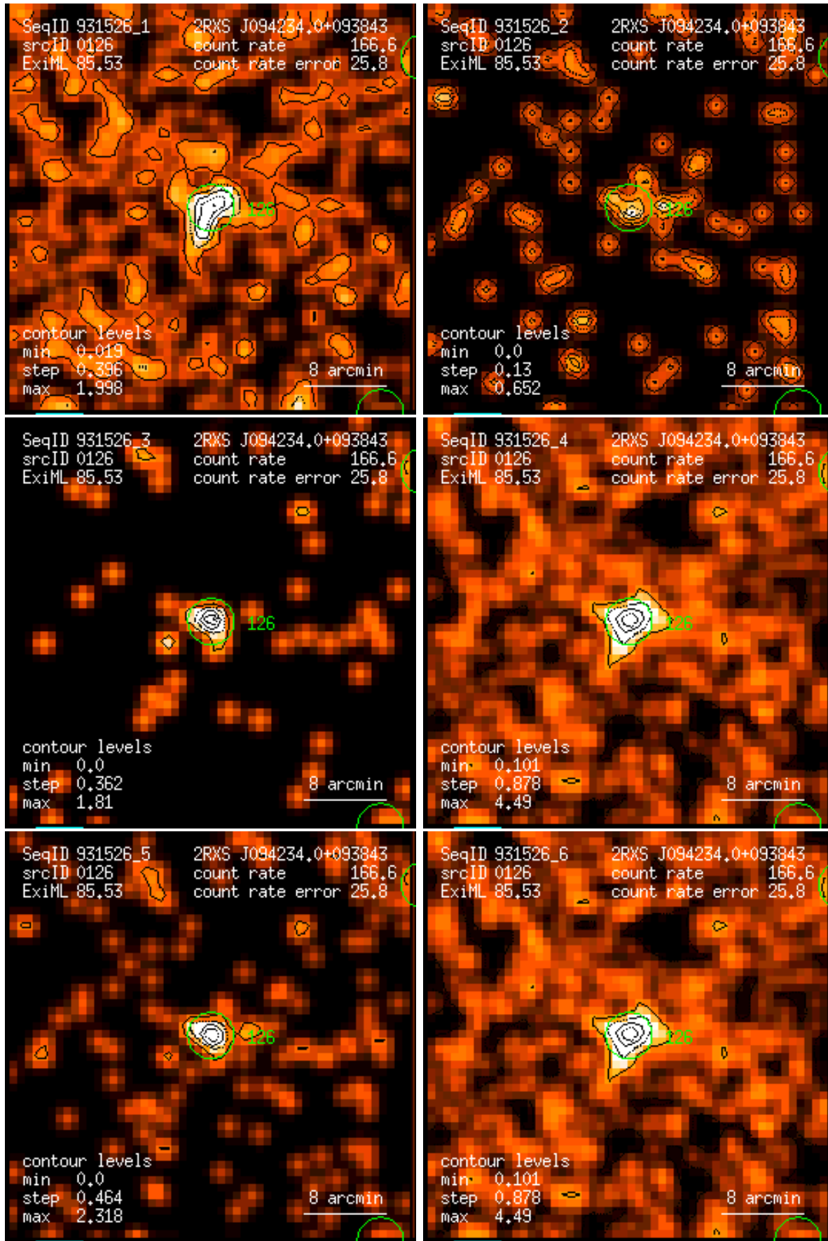
Figure 126: RASS 931526: detection 0126: band rate images, Gaussian filter: (1) PSPC channels 11 – 41, (2) 52 – 90, (3) 91 – 201, (4) 11 – 235, (5) 52 – 201, (6) 11 – 201. Broad band rates in counts/ks. Band rate contour levels in counts/ks/arcmin 2 .
