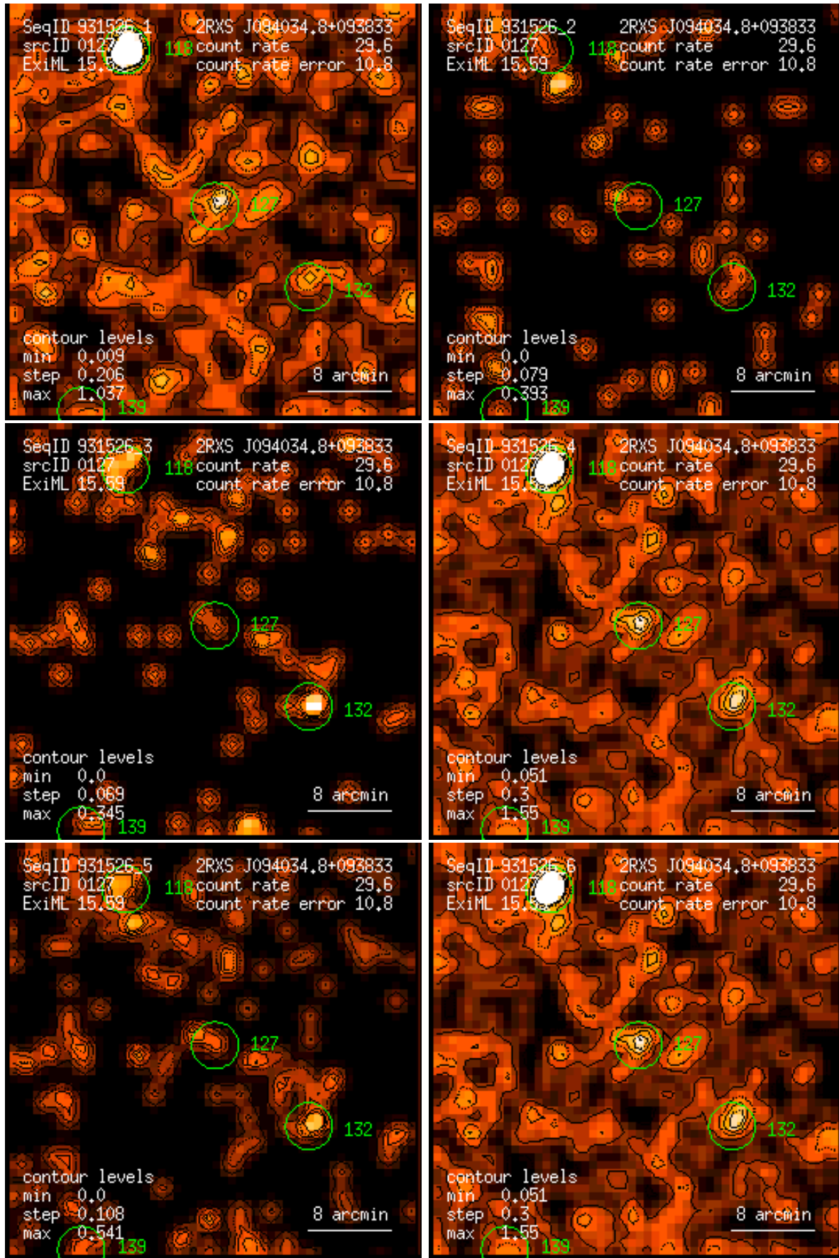
Figure 127: RASS 931526: detection 0127: band rate images, Gaussian filter: (1) PSPC channels 11 – 41, (2) 52 – 90, (3) 91 – 201, (4) 11 – 235, (5) 52 – 201, (6) 11 – 201. Broad band rates in counts/ks. Band rate contour levels in counts/ks/arcmin 2 .
