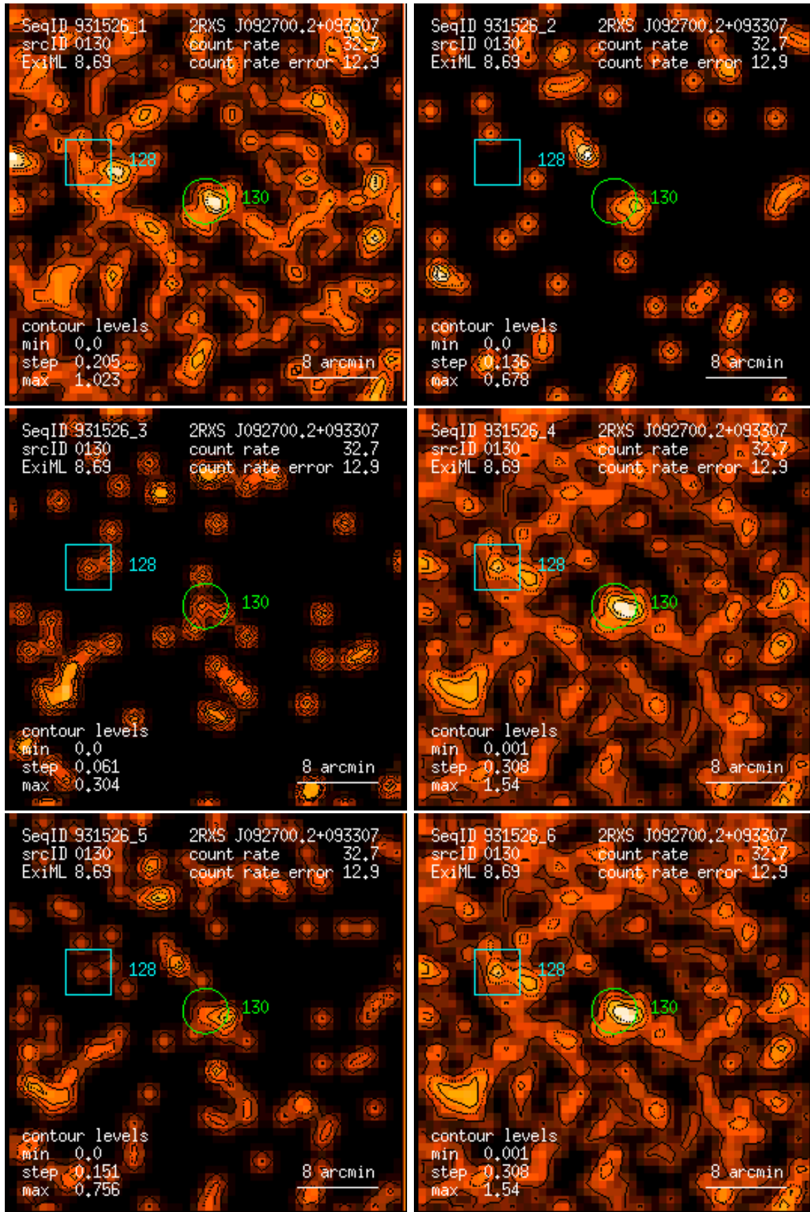
Figure 130: RASS 931526: detection 0130: band rate images, Gaussian filter: (1) PSPC channels 11 – 41, (2) 52 – 90, (3) 91 – 201, (4) 11 – 235, (5) 52 – 201, (6) 11 – 201. Broad band rates in counts/ks. Band rate contour levels in counts/ks/arcmin 2 .
