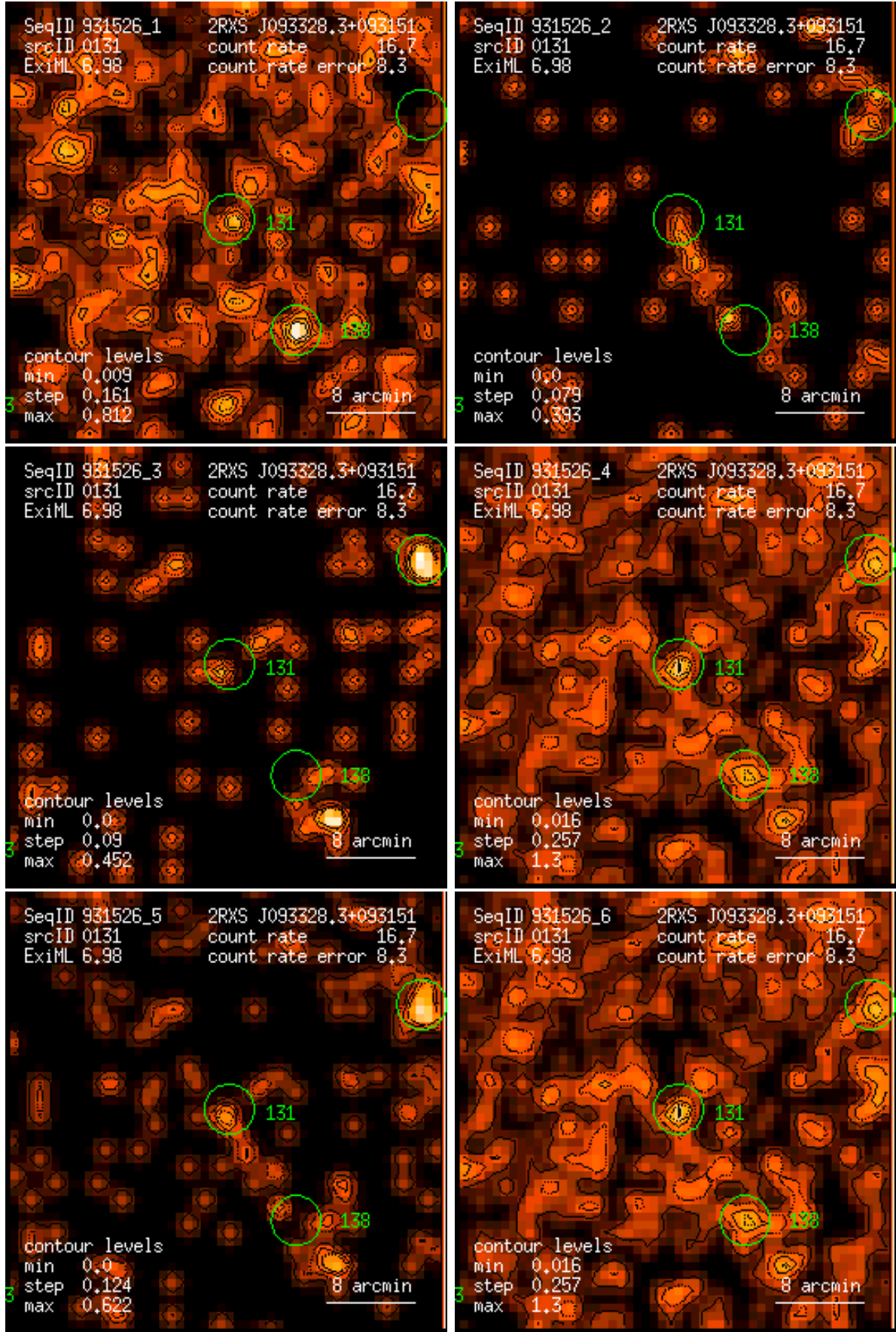
Figure 131: RASS 931526: detection 0131: band rate images, Gaussian filter: (1) PSPC channels 11 – 41, (2) 52 – 90, (3) 91 – 201, (4) 11 – 235, (5) 52 – 201, (6) 11 – 201. Broad band rates in counts/ks. Band rate contour levels in counts/ks/arcmin 2 .
