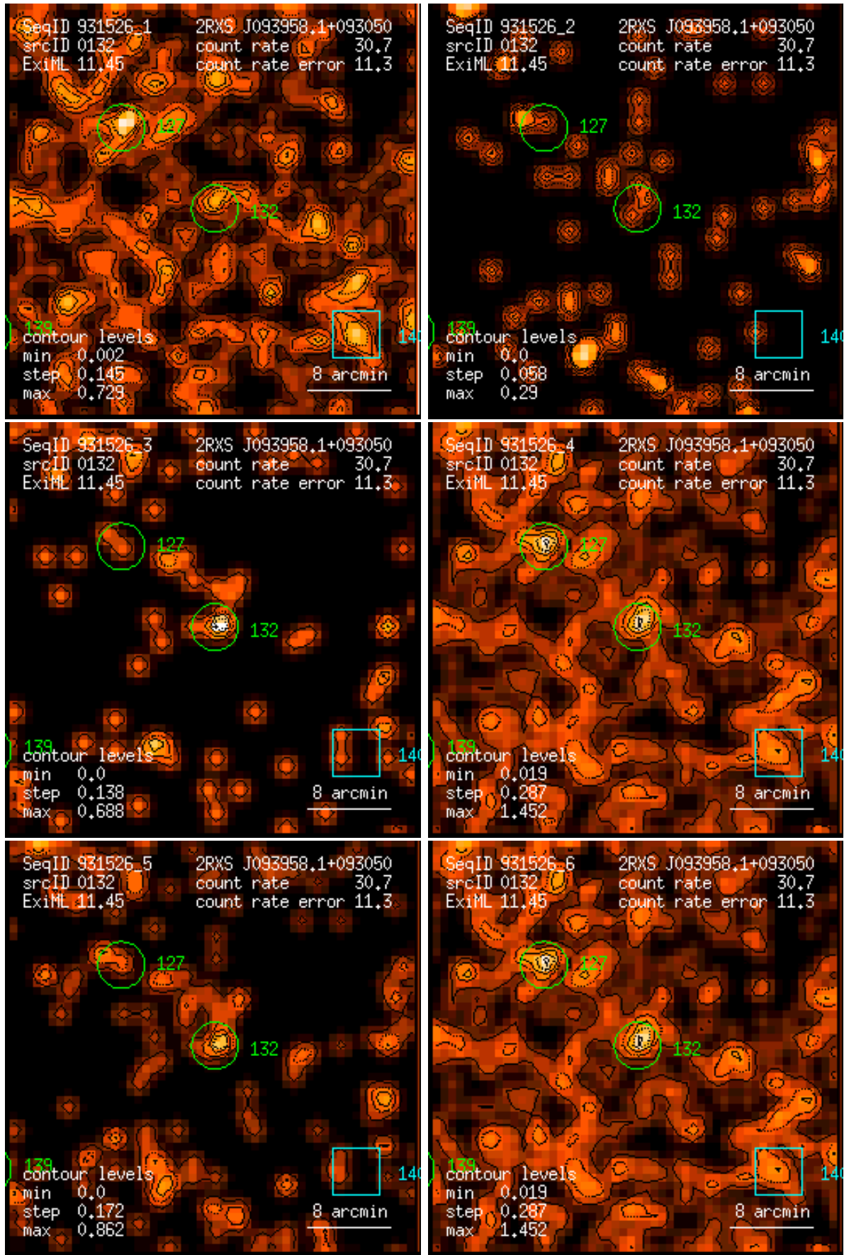
Figure 132: RASS 931526: detection 0132: band rate images, Gaussian filter: (1) PSPC channels 11 – 41, (2) 52 – 90, (3) 91 – 201, (4) 11 – 235, (5) 52 – 201, (6) 11 – 201. Broad band rates in counts/ks. Band rate contour levels in counts/ks/arcmin 2 .
