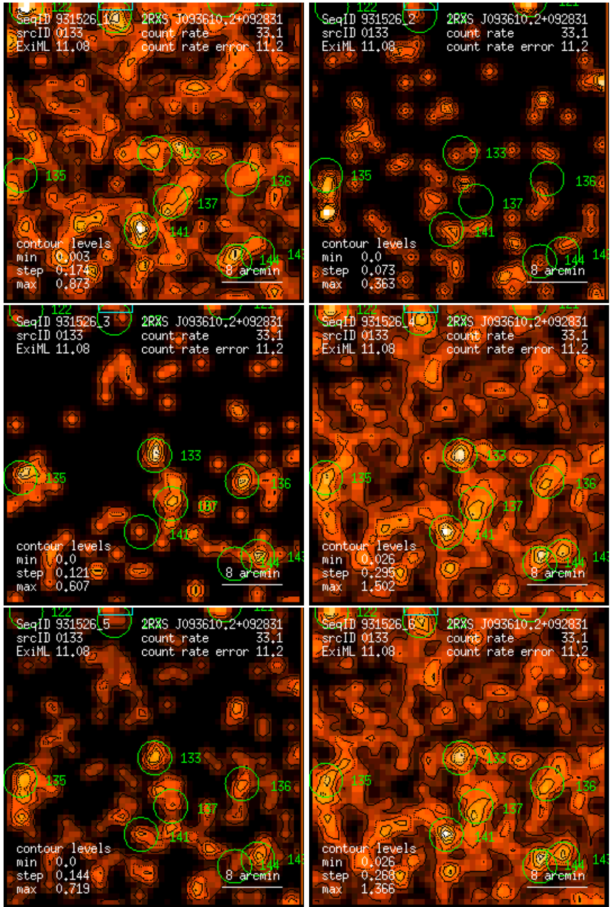
Figure 133: RASS 931526: detection 0133: band rate images, Gaussian filter: (1) PSPC channels 11 – 41, (2) 52 – 90, (3) 91 – 201, (4) 11 – 235, (5) 52 – 201, (6) 11 – 201. Broad band rates in counts/ks. Band rate contour levels in counts/ks/arcmin 2 .
