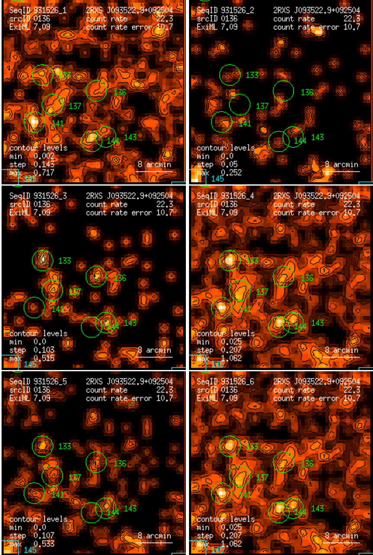
Figure 136: RASS 931526: detection 0136: band rate images, Gaussian filter: (1) PSPC channels 11 – 41, (2) 52 – 90, (3) 91 – 201, (4) 11 – 235, (5) 52 – 201, (6) 11 – 201. Broad band rates in counts/ks. Band rate contour levels in counts/ks/arcmin 2 .
