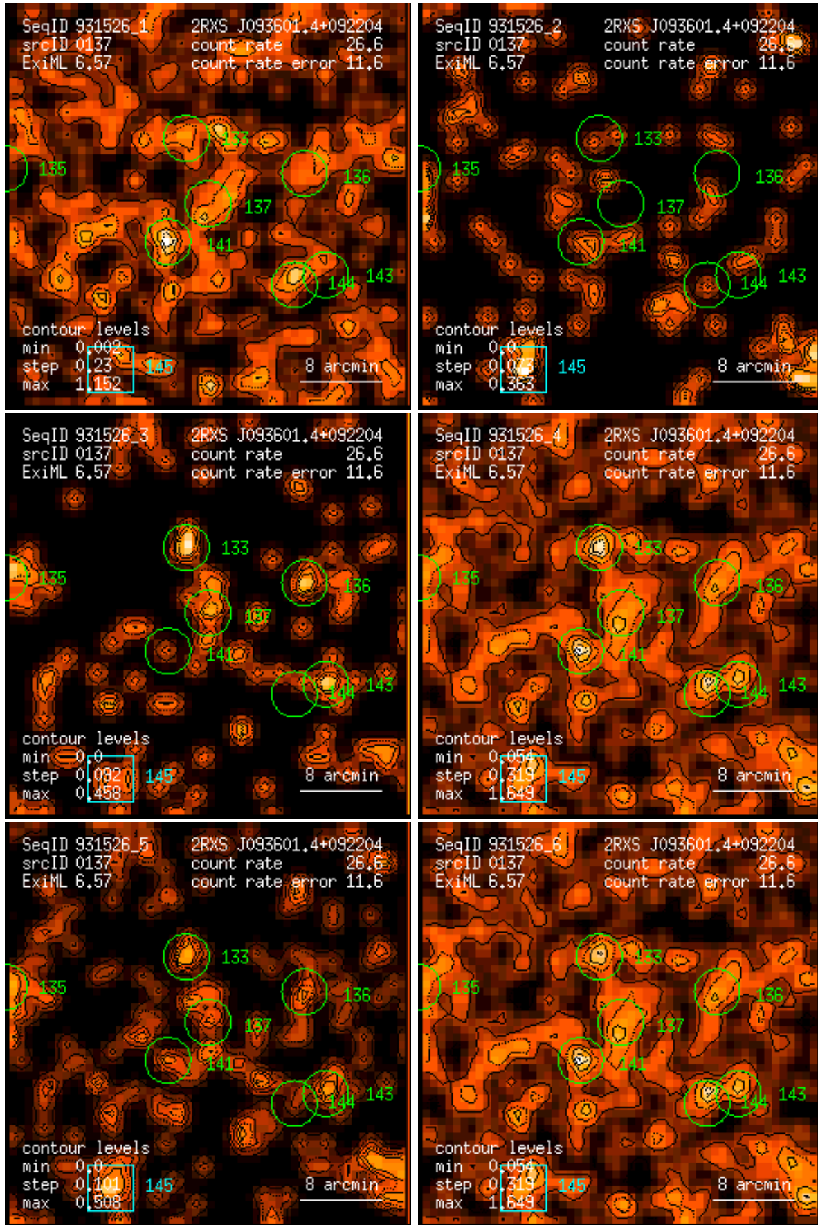
Figure 137: RASS 931526: detection 0137: band rate images, Gaussian filter: (1) PSPC channels 11 – 41, (2) 52 – 90, (3) 91 – 201, (4) 11 – 235, (5) 52 – 201, (6) 11 – 201. Broad band rates in counts/ks. Band rate contour levels in counts/ks/arcmin 2 .
