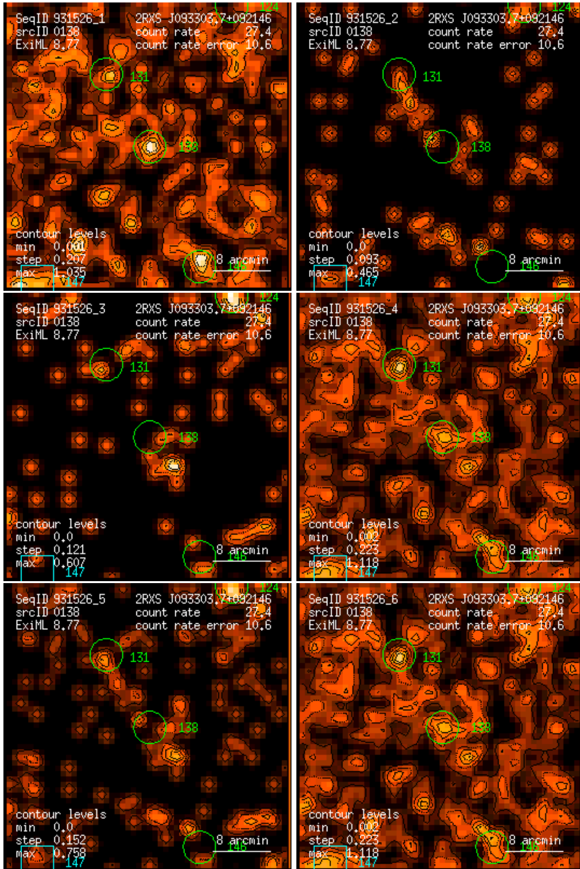
Figure 138: RASS 931526: detection 0138: band rate images, Gaussian filter: (1) PSPC channels 11 – 41, (2) 52 – 90, (3) 91 – 201, (4) 11 – 235, (5) 52 – 201, (6) 11 – 201. Broad band rates in counts/ks. Band rate contour levels in counts/ks/arcmin 2 .
