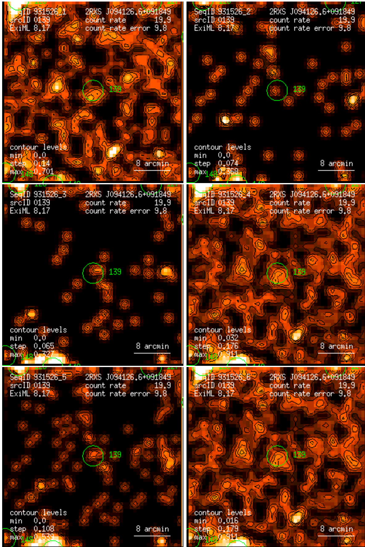
Figure 139: RASS 931526: detection 0139: band rate images, Gaussian filter: (1) PSPC channels 11 – 41, (2) 52 – 90, (3) 91 – 201, (4) 11 – 235, (5) 52 – 201, (6) 11 – 201. Broad band rates in counts/ks. Band rate contour levels in counts/ks/arcmin 2 .
