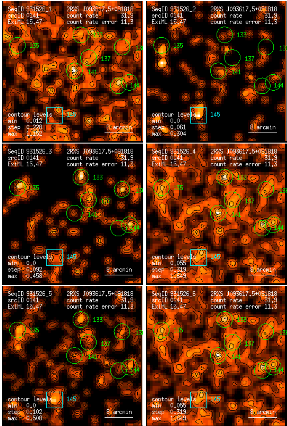
Figure 141: RASS 931526: detection 0141: band rate images, Gaussian filter: (1) PSPC channels 11 – 41, (2) 52 – 90, (3) 91 – 201, (4) 11 – 235, (5) 52 – 201, (6) 11 – 201. Broad band rates in counts/ks. Band rate contour levels in counts/ks/arcmin 2 .
