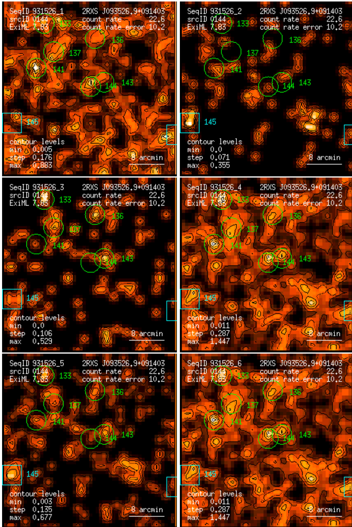
Figure 144: RASS 931526: detection 0144: band rate images, Gaussian filter: (1) PSPC channels 11 – 41, (2) 52 – 90, (3) 91 – 201, (4) 11 – 235, (5) 52 – 201, (6) 11 – 201. Broad band rates in counts/ks. Band rate contour levels in counts/ks/arcmin 2 .
