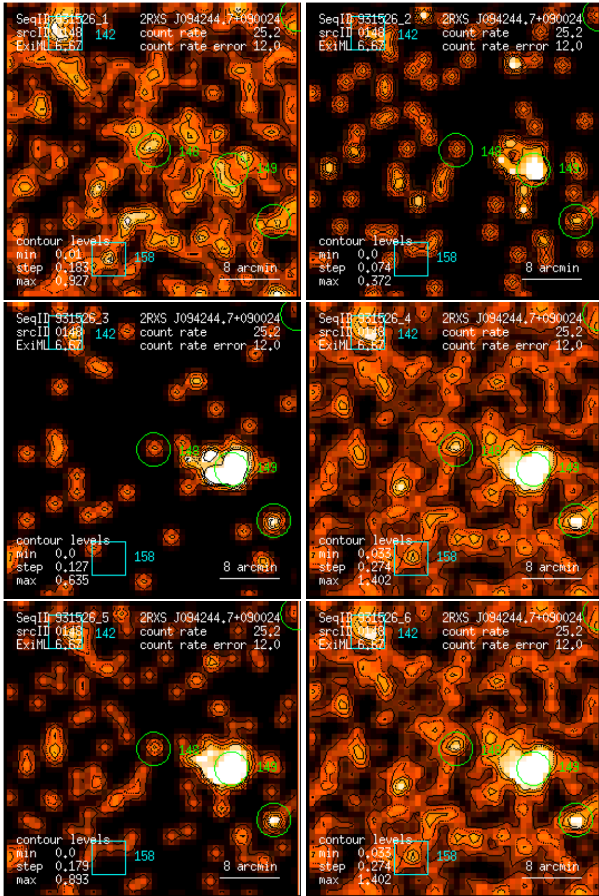
Figure 148: RASS 931526: detection 0148: band rate images, Gaussian filter: (1) PSPC channels 11 – 41, (2) 52 – 90, (3) 91 – 201, (4) 11 – 235, (5) 52 – 201, (6) 11 – 201. Broad band rates in counts/ks. Band rate contour levels in counts/ks/arcmin 2 .
