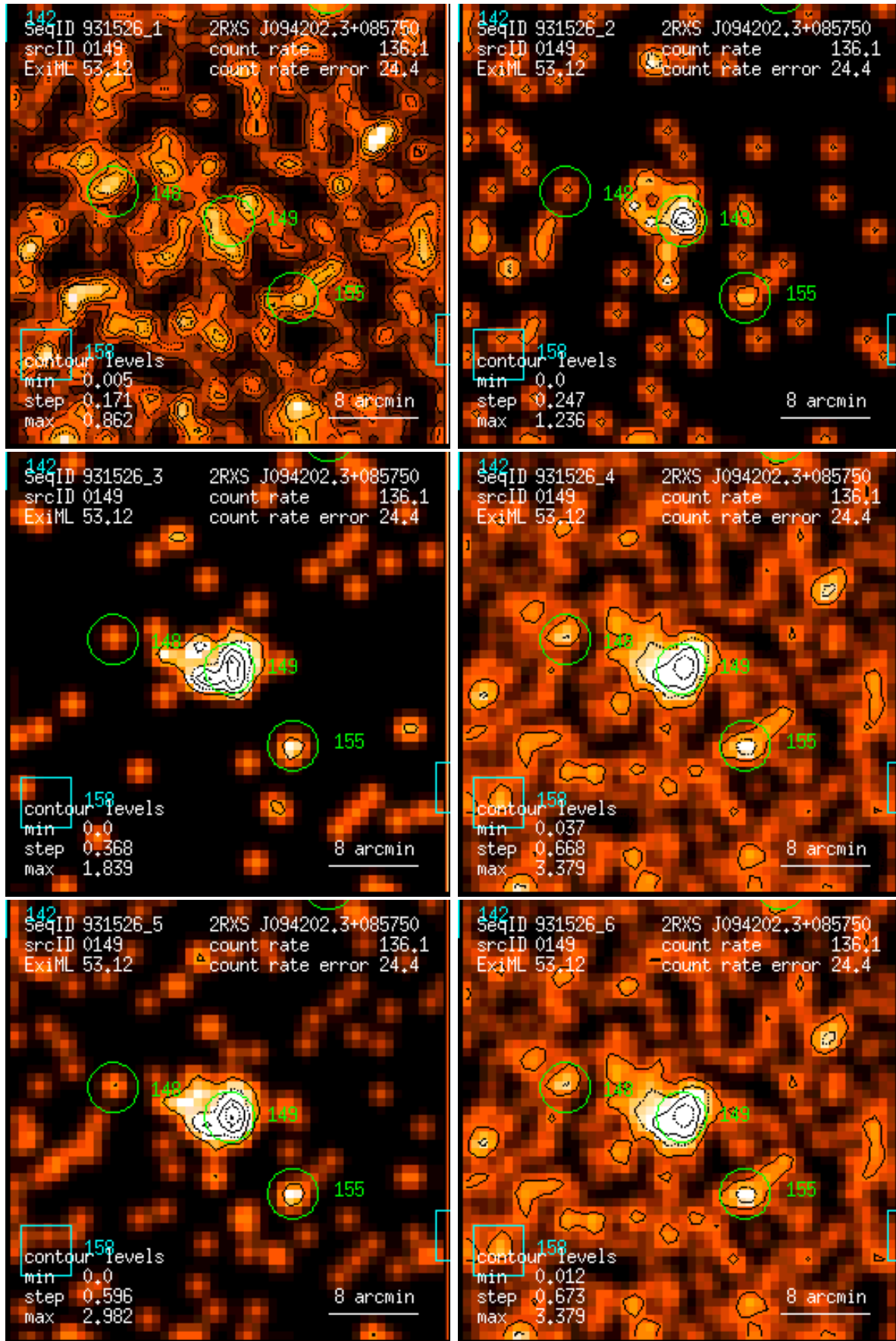
Figure 149: RASS 931526: detection 0149: band rate images, Gaussian filter: (1) PSPC channels 11 – 41, (2) 52 – 90, (3) 91 – 201, (4) 11 – 235, (5) 52 – 201, (6) 11 – 201. Broad band rates in counts/ks. Band rate contour levels in counts/ks/arcmin 2 .
