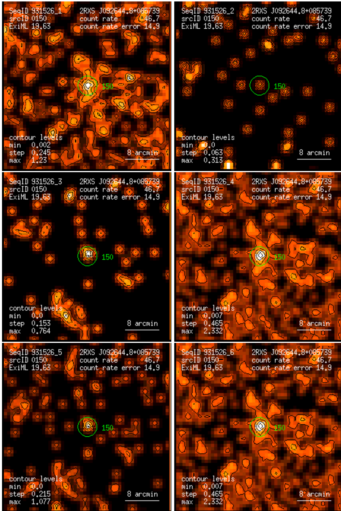
Figure 150: RASS 931526: detection 0150: band rate images, Gaussian filter: (1) PSPC channels 11 – 41, (2) 52 – 90, (3) 91 – 201, (4) 11 – 235, (5) 52 – 201, (6) 11 – 201. Broad band rates in counts/ks. Band rate contour levels in counts/ks/arcmin 2 .
