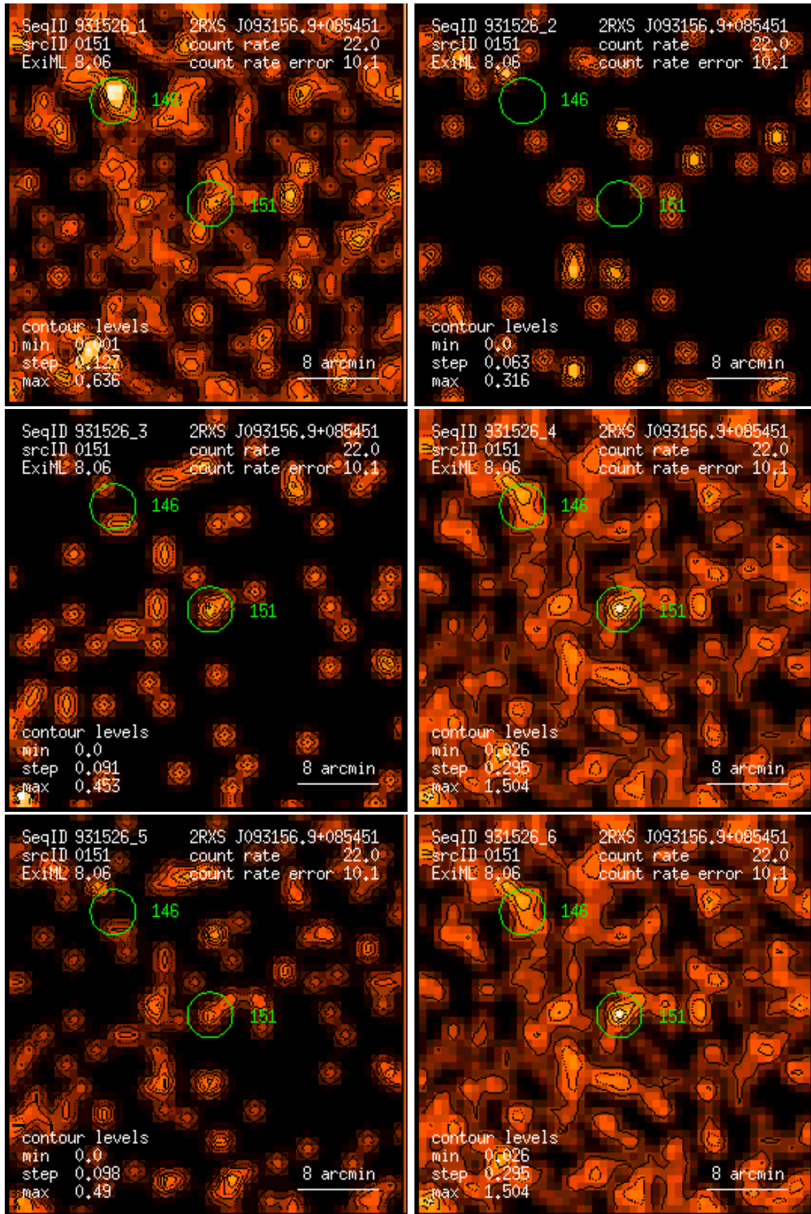
Figure 151: RASS 931526: detection 0151: band rate images, Gaussian filter: (1) PSPC channels 11 – 41, (2) 52 – 90, (3) 91 – 201, (4) 11 – 235, (5) 52 – 201, (6) 11 – 201. Broad band rates in counts/ks. Band rate contour levels in counts/ks/arcmin 2 .
