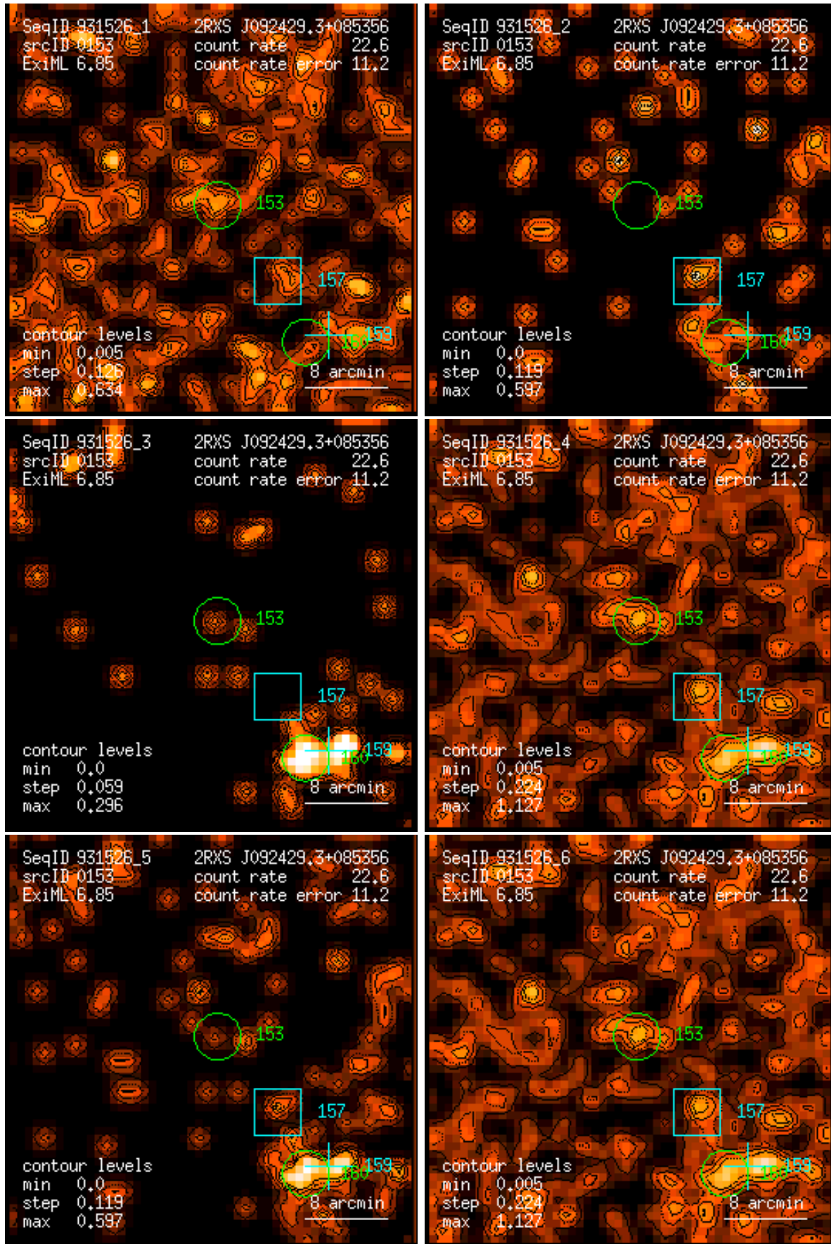
Figure 153: RASS 931526: detection 0153: band rate images, Gaussian filter: (1) PSPC channels 11 – 41, (2) 52 – 90, (3) 91 – 201, (4) 11 – 235, (5) 52 – 201, (6) 11 – 201. Broad band rates in counts/ks. Band rate contour levels in counts/ks/arcmin 2 .
