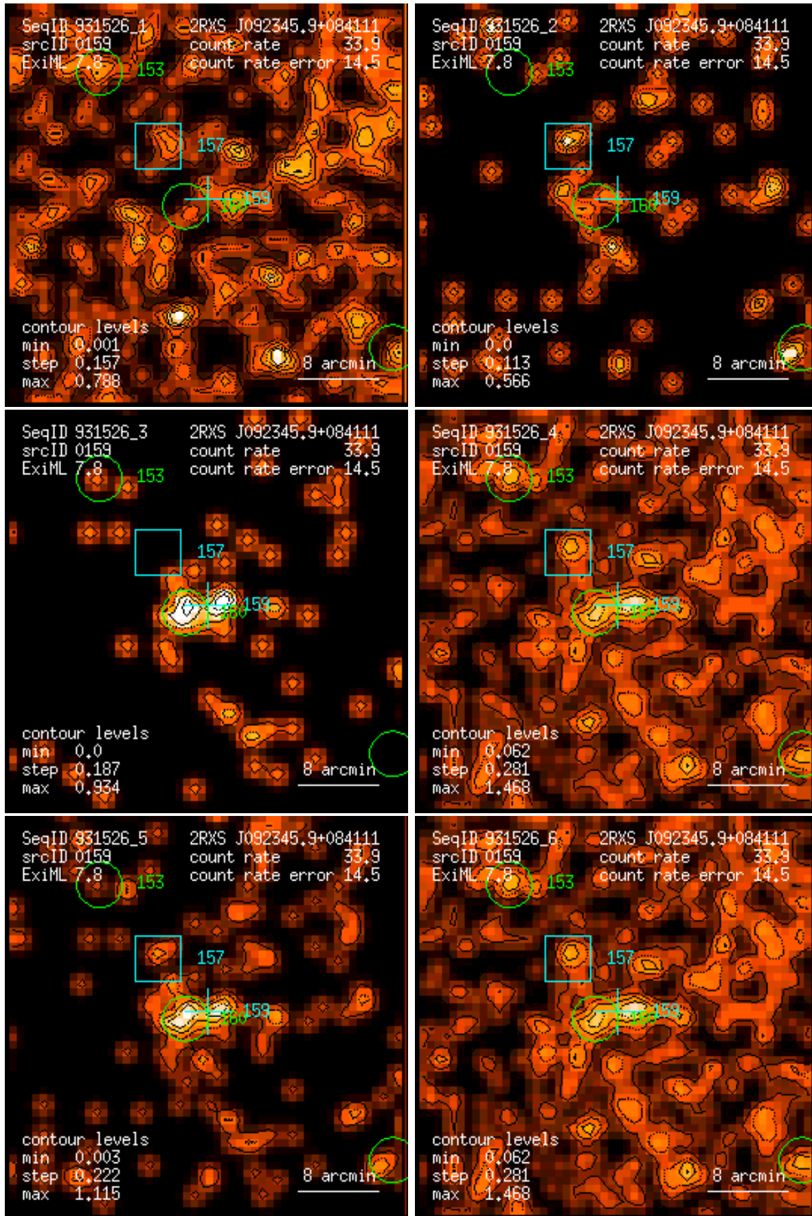
Figure 159: RASS 931526: detection 0159: band rate images, Gaussian filter: (1) PSPC channels 11 – 41, (2) 52 – 90, (3) 91 – 201, (4) 11 – 235, (5) 52 – 201, (6) 11 – 201. Broad band rates in counts/ks. Band rate contour levels in counts/ks/arcmin 2 .
