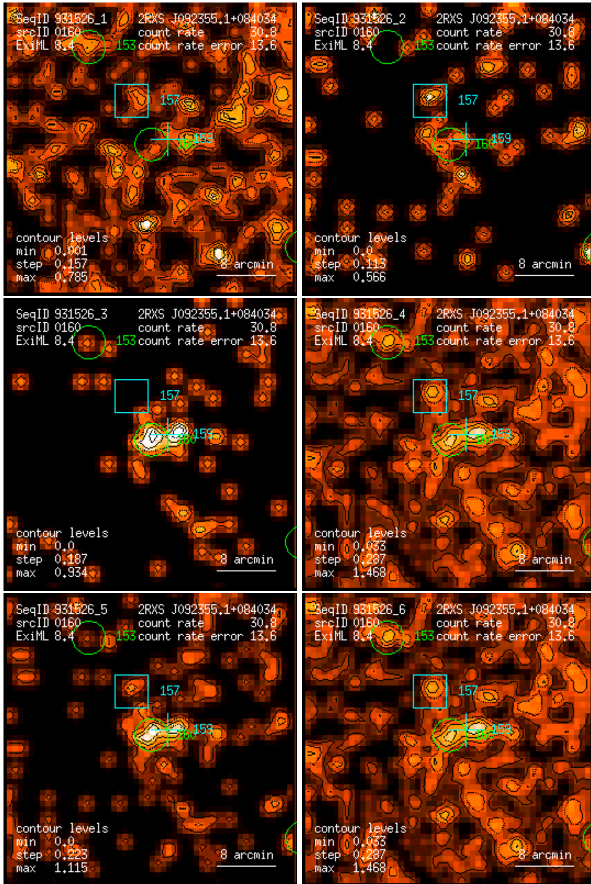
Figure 160: RASS 931526: detection 0160: band rate images, Gaussian filter: (1) PSPC channels 11 – 41, (2) 52 – 90, (3) 91 – 201, (4) 11 – 235, (5) 52 – 201, (6) 11 – 201. Broad band rates in counts/ks. Band rate contour levels in counts/ks/arcmin 2 .
