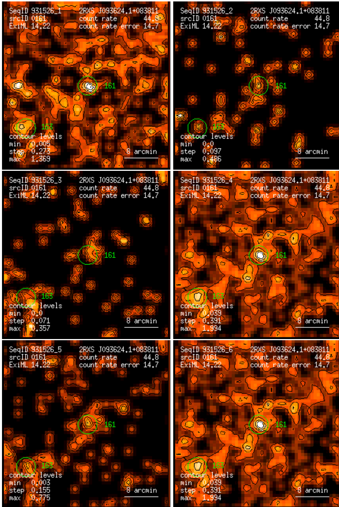
Figure 161: RASS 931526: detection 0161: band rate images, Gaussian filter: (1) PSPC channels 11 – 41, (2) 52 – 90, (3) 91 – 201, (4) 11 – 235, (5) 52 – 201, (6) 11 – 201. Broad band rates in counts/ks. Band rate contour levels in counts/ks/arcmin 2 .
