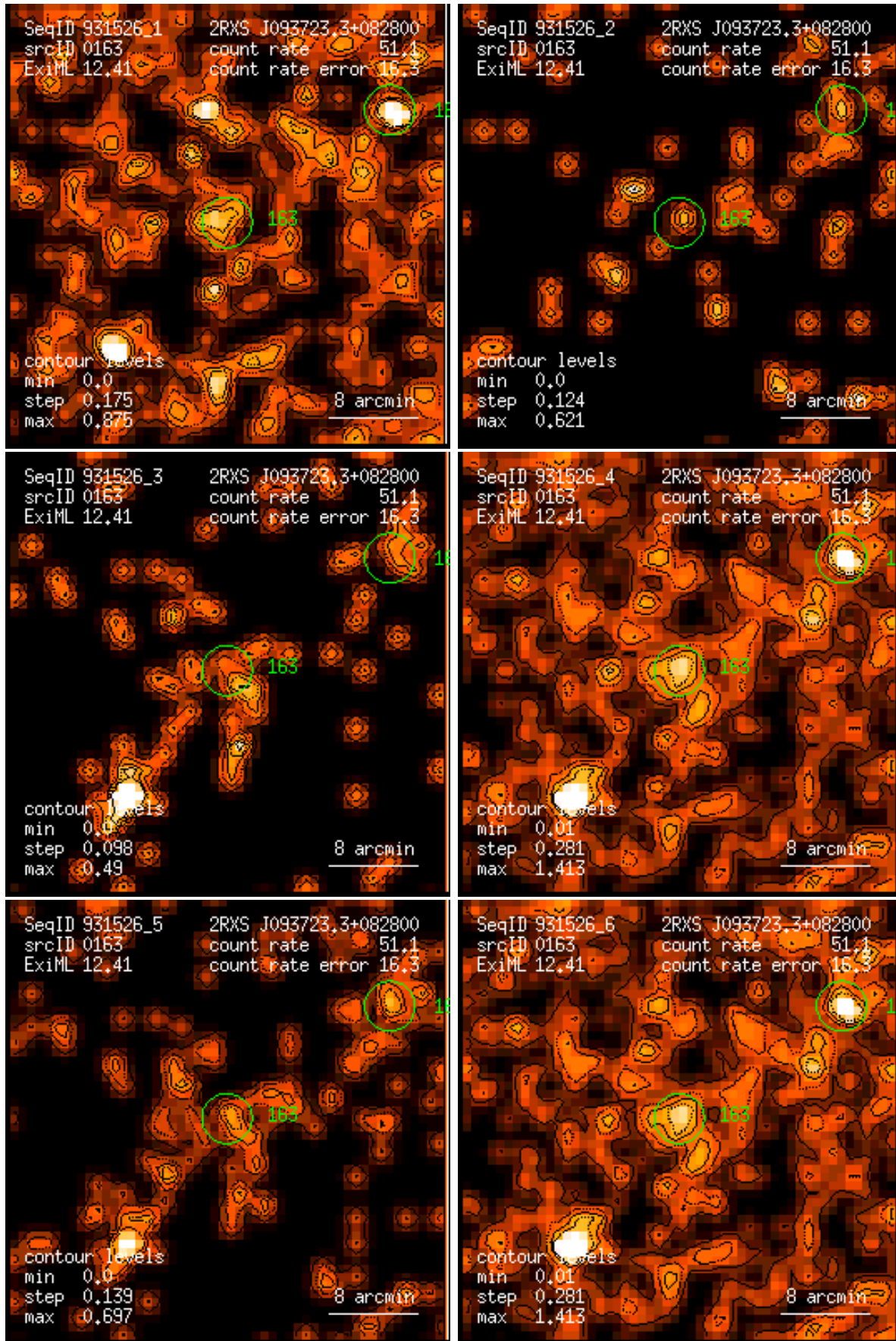
Figure 163: RASS 931526: detection 0163: band rate images, Gaussian filter: (1) PSPC channels 11 – 41, (2) 52 – 90, (3) 91 – 201, (4) 11 – 235, (5) 52 – 201, (6) 11 – 201. Broad band rates in counts/ks. Band rate contour levels in counts/ks/arcmin 2 .
