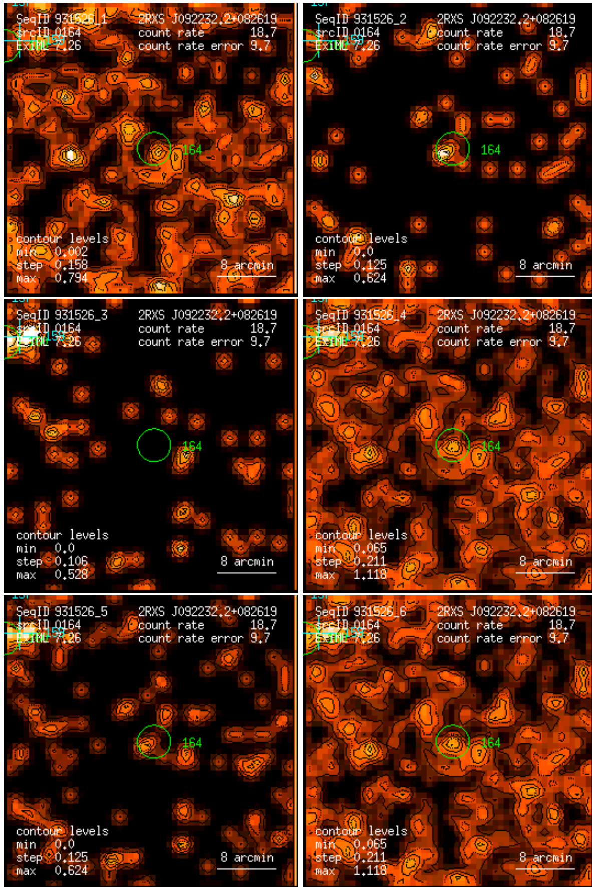
Figure 164: RASS 931526: detection 0164: band rate images, Gaussian filter: (1) PSPC channels 11 – 41, (2) 52 – 90, (3) 91 – 201, (4) 11 – 235, (5) 52 – 201, (6) 11 – 201. Broad band rates in counts/ks. Band rate contour levels in counts/ks/arcmin 2 .
