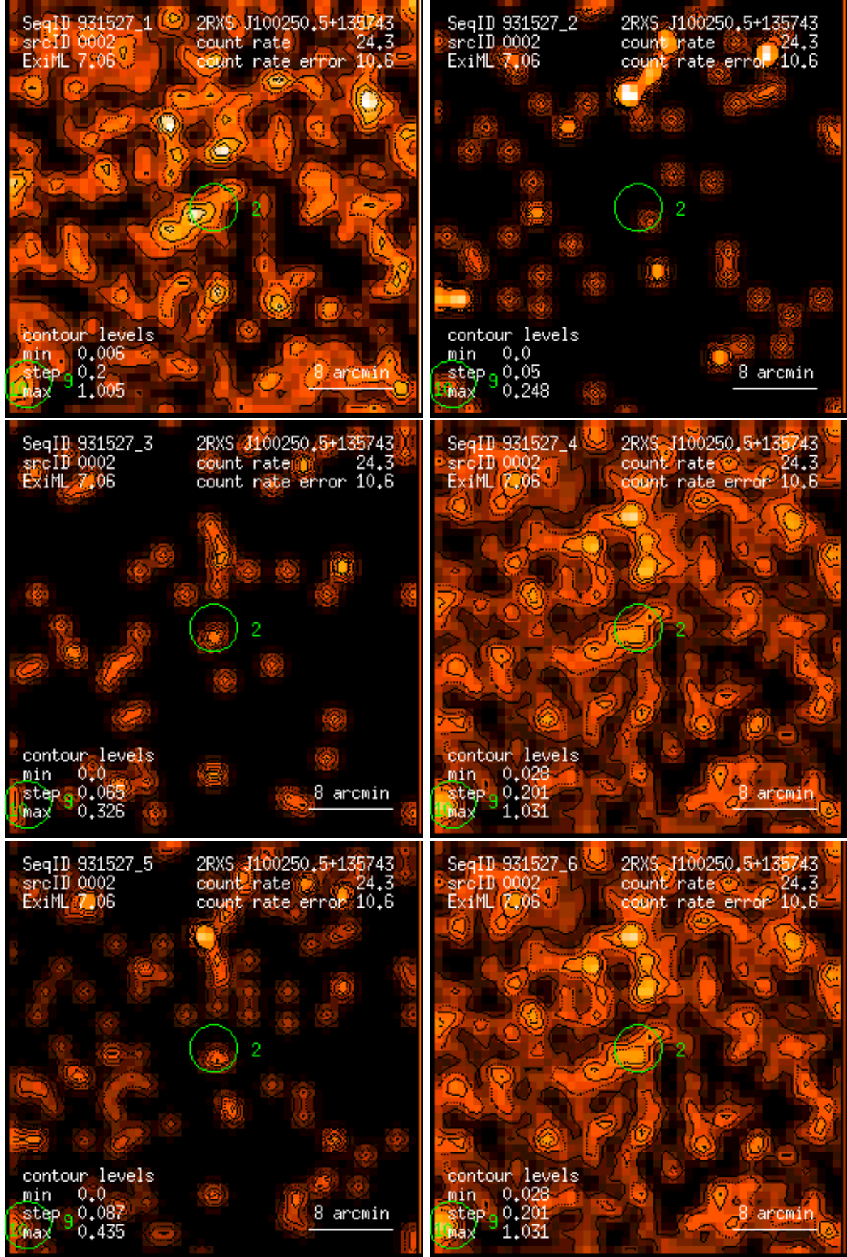
Figure 2: RASS 931527: detection 0002: band rate images, Gaussian filter: (1) PSPC channels 11 – 41, (2) 52 – 90, (3) 91 – 201, (4) 11 – 235, (5) 52 – 201, (6) 11 – 201. Broad band rates in counts/ks. Band rate contour levels in counts/ks/arcmin 2 .
