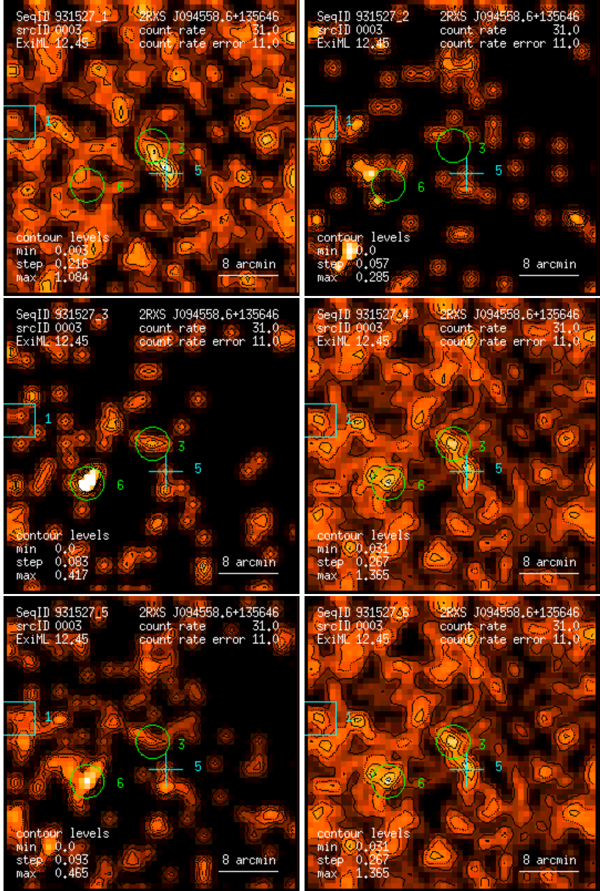
Figure 3: RASS 931527: detection 0003: band rate images, Gaussian filter: (1) PSPC channels 11 – 41, (2) 52 – 90, (3) 91 – 201, (4) 11 – 235, (5) 52 – 201, (6) 11 – 201. Broad band rates in counts/ks. Band rate contour levels in counts/ks/arcmin 2 .
