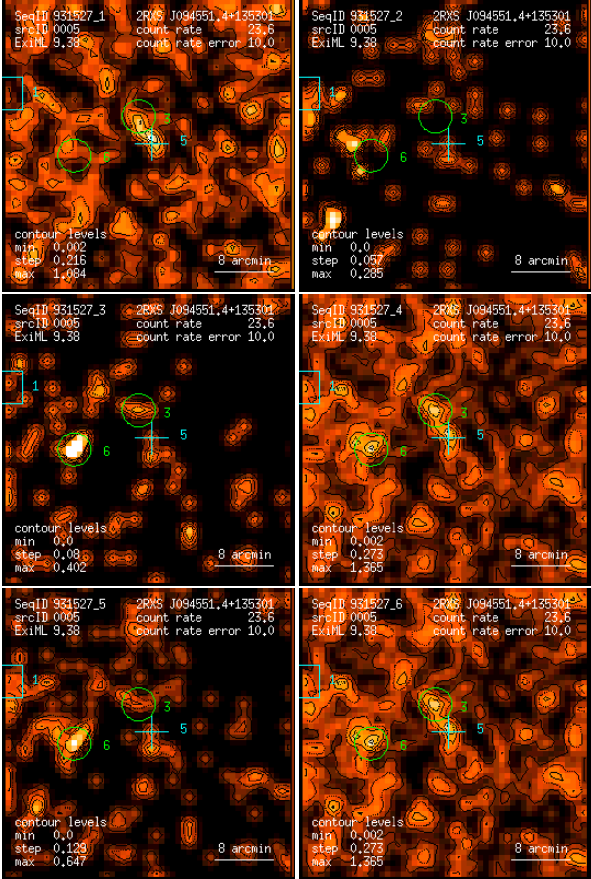
Figure 5: RASS 931527: detection 0005: band rate images, Gaussian filter: (1) PSPC channels 11 – 41, (2) 52 – 90, (3) 91 – 201, (4) 11 – 235, (5) 52 – 201, (6) 11 – 201. Broad band rates in counts/ks. Band rate contour levels in counts/ks/arcmin 2 .
