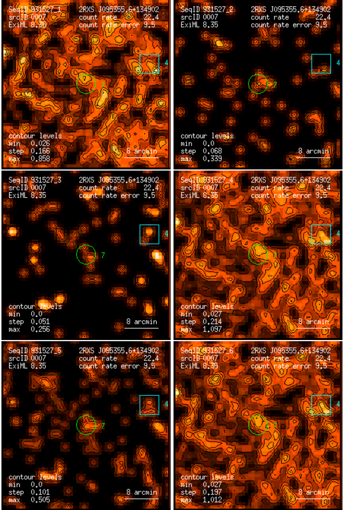
Figure 7: RASS 931527: detection 0007: band rate images, Gaussian filter: (1) PSPC channels 11 – 41, (2) 52 – 90, (3) 91 – 201, (4) 11 – 235, (5) 52 – 201, (6) 11 – 201. Broad band rates in counts/ks. Band rate contour levels in counts/ks/arcmin 2 .
