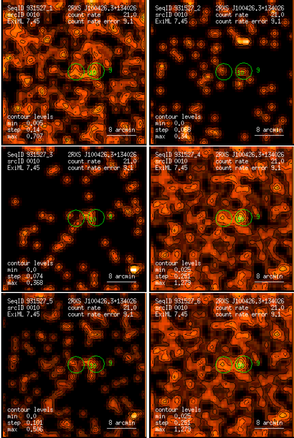
Figure 10: RASS 931527: detection 0010: band rate images, Gaussian filter: (1) PSPC channels 11 – 41, (2) 52 – 90, (3) 91 – 201, (4) 11 – 235, (5) 52 – 201, (6) 11 – 201. Broad band rates in counts/ks. Band rate contour levels in counts/ks/arcmin 2 .
