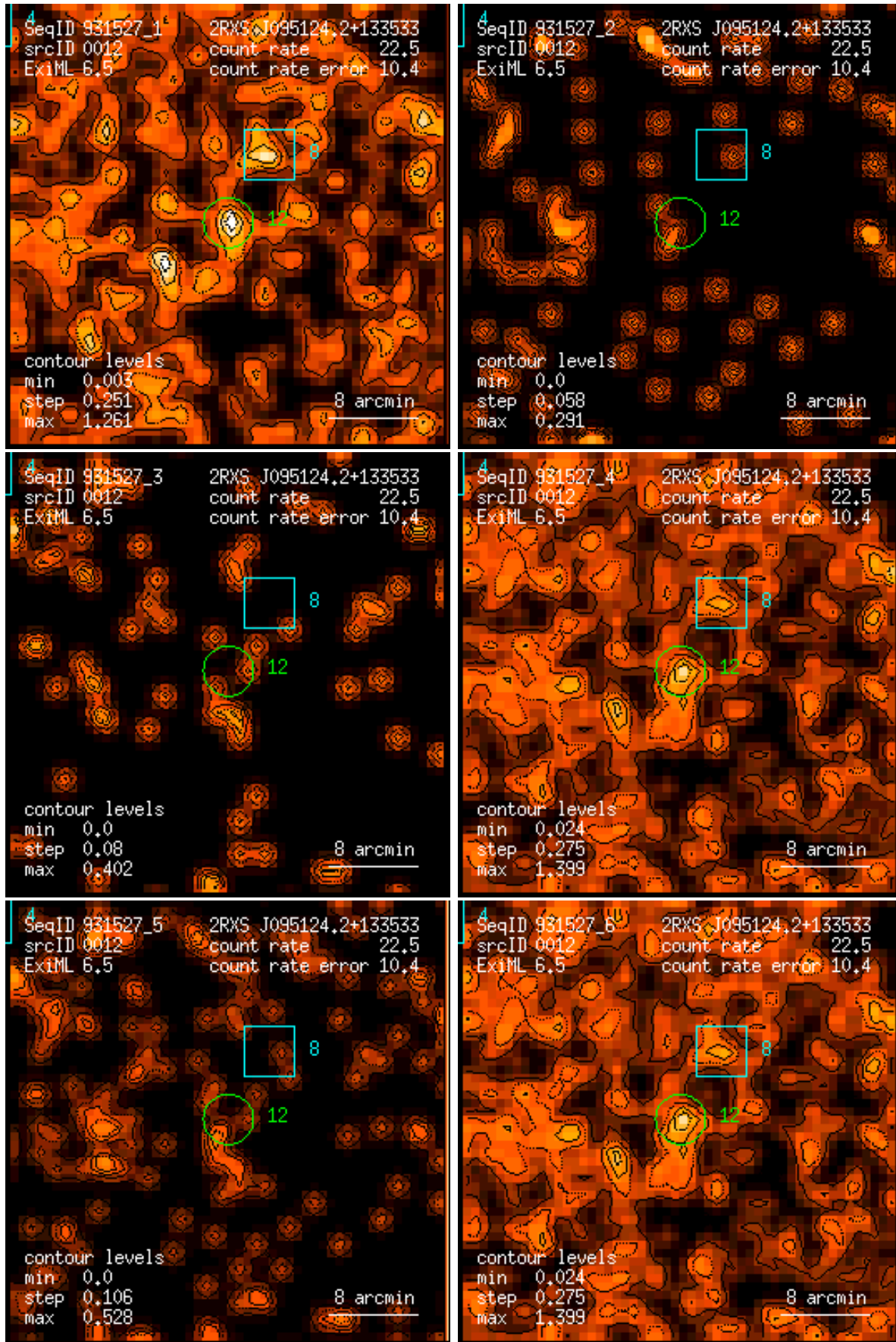
Figure 12: RASS 931527: detection 0012: band rate images, Gaussian filter: (1) PSPC channels 11 – 41, (2) 52 – 90, (3) 91 – 201, (4) 11 – 235, (5) 52 – 201, (6) 11 – 201. Broad band rates in counts/ks. Band rate contour levels in counts/ks/arcmin 2 .
