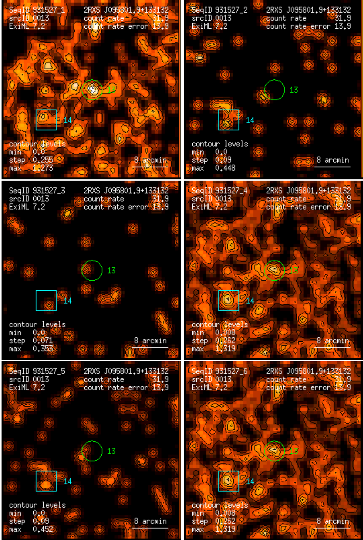
Figure 13: RASS 931527: detection 0013: band rate images, Gaussian filter: (1) PSPC channels 11 – 41, (2) 52 – 90, (3) 91 – 201, (4) 11 – 235, (5) 52 – 201, (6) 11 – 201. Broad band rates in counts/ks. Band rate contour levels in counts/ks/arcmin 2 .
