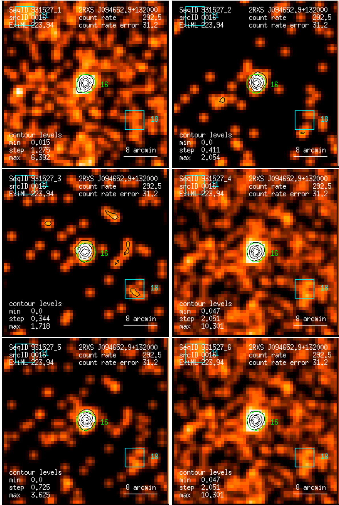
Figure 16: RASS 931527: detection 0016: band rate images, Gaussian filter: (1) PSPC channels 11 – 41, (2) 52 – 90, (3) 91 – 201, (4) 11 – 235, (5) 52 – 201, (6) 11 – 201. Broad band rates in counts/ks. Band rate contour levels in counts/ks/arcmin 2 .
