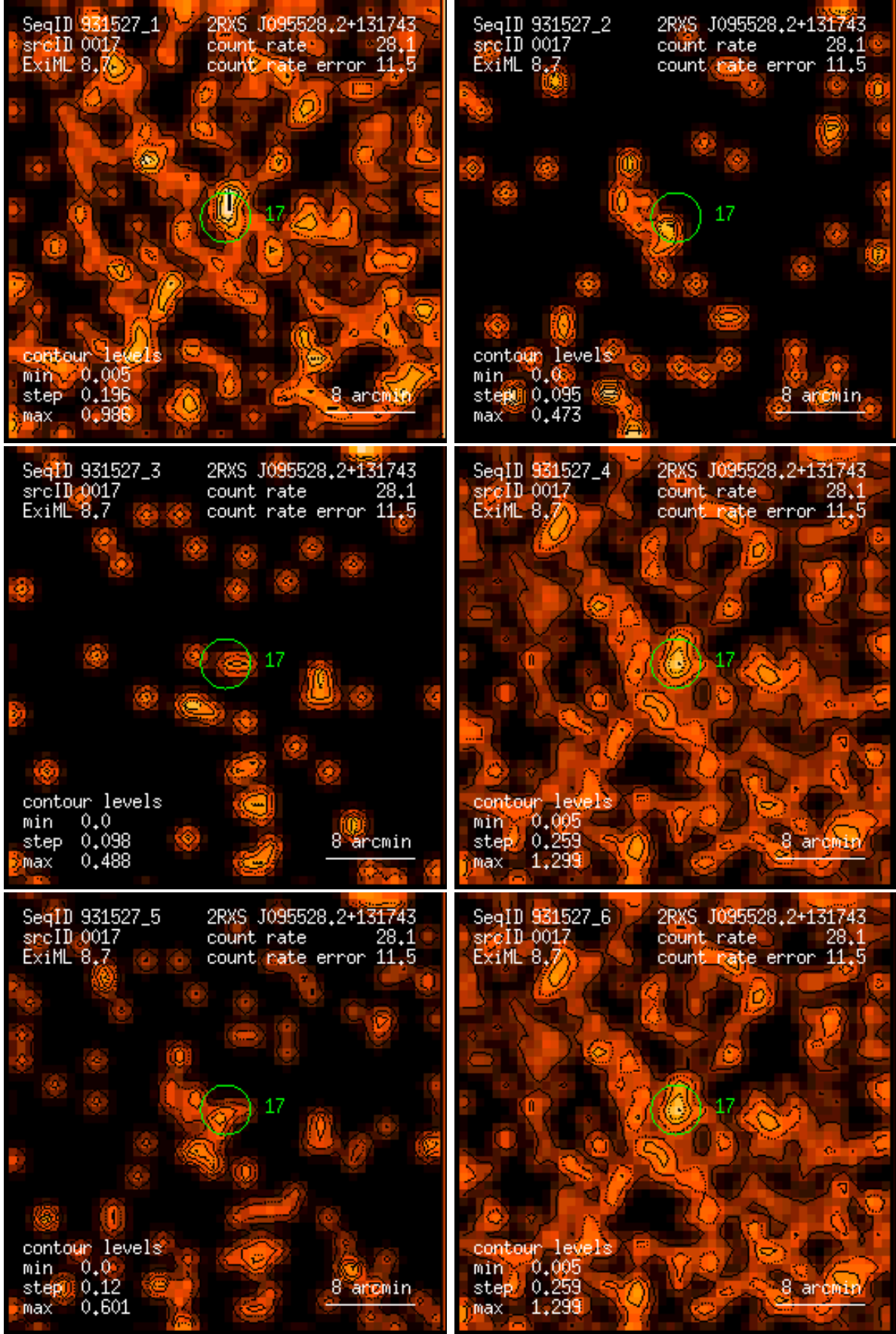
Figure 17: RASS 931527: detection 0017: band rate images, Gaussian filter: (1) PSPC channels 11 – 41, (2) 52 – 90, (3) 91 – 201, (4) 11 – 235, (5) 52 – 201, (6) 11 – 201. Broad band rates in counts/ks. Band rate contour levels in counts/ks/arcmin 2 .
