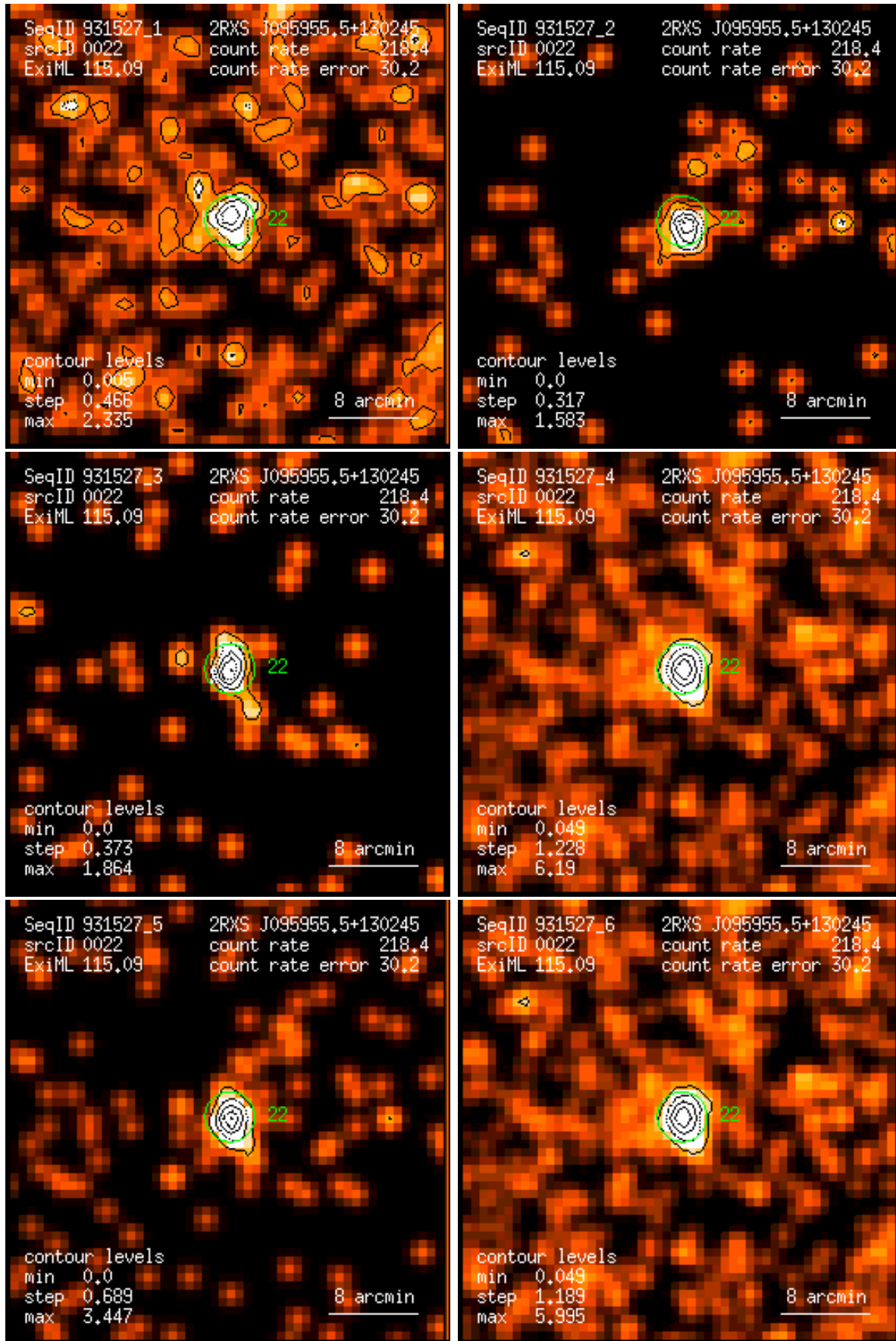
Figure 22: RASS 931527: detection 0022: band rate images, Gaussian filter: (1) PSPC channels 11 – 41, (2) 52 – 90, (3) 91 – 201, (4) 11 – 235, (5) 52 – 201, (6) 11 – 201. Broad band rates in counts/ks. Band rate contour levels in counts/ks/arcmin 2 .
