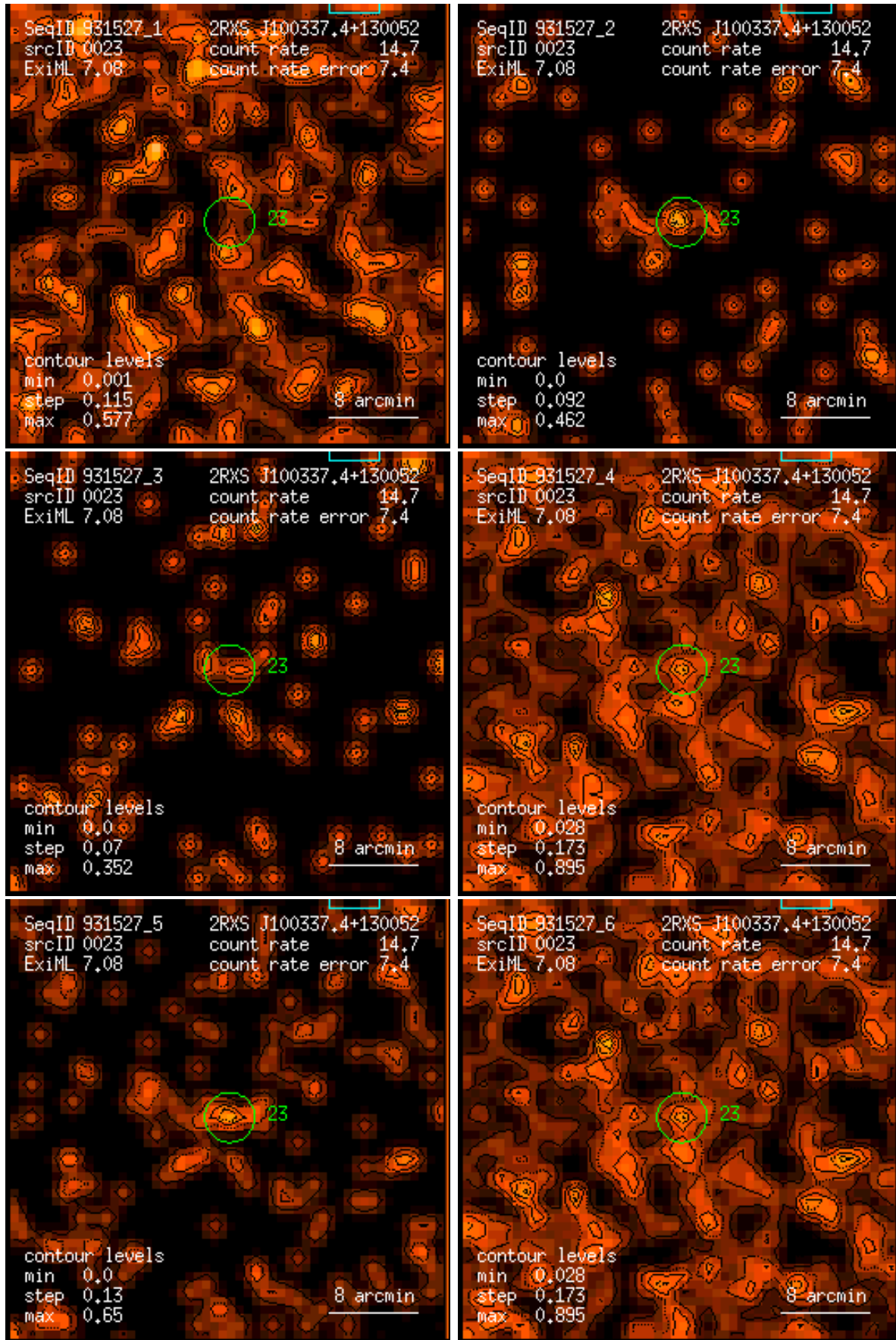
Figure 23: RASS 931527: detection 0023: band rate images, Gaussian filter: (1) PSPC channels 11 – 41, (2) 52 – 90, (3) 91 – 201, (4) 11 – 235, (5) 52 – 201, (6) 11 – 201. Broad band rates in counts/ks. Band rate contour levels in counts/ks/arcmin 2 .
